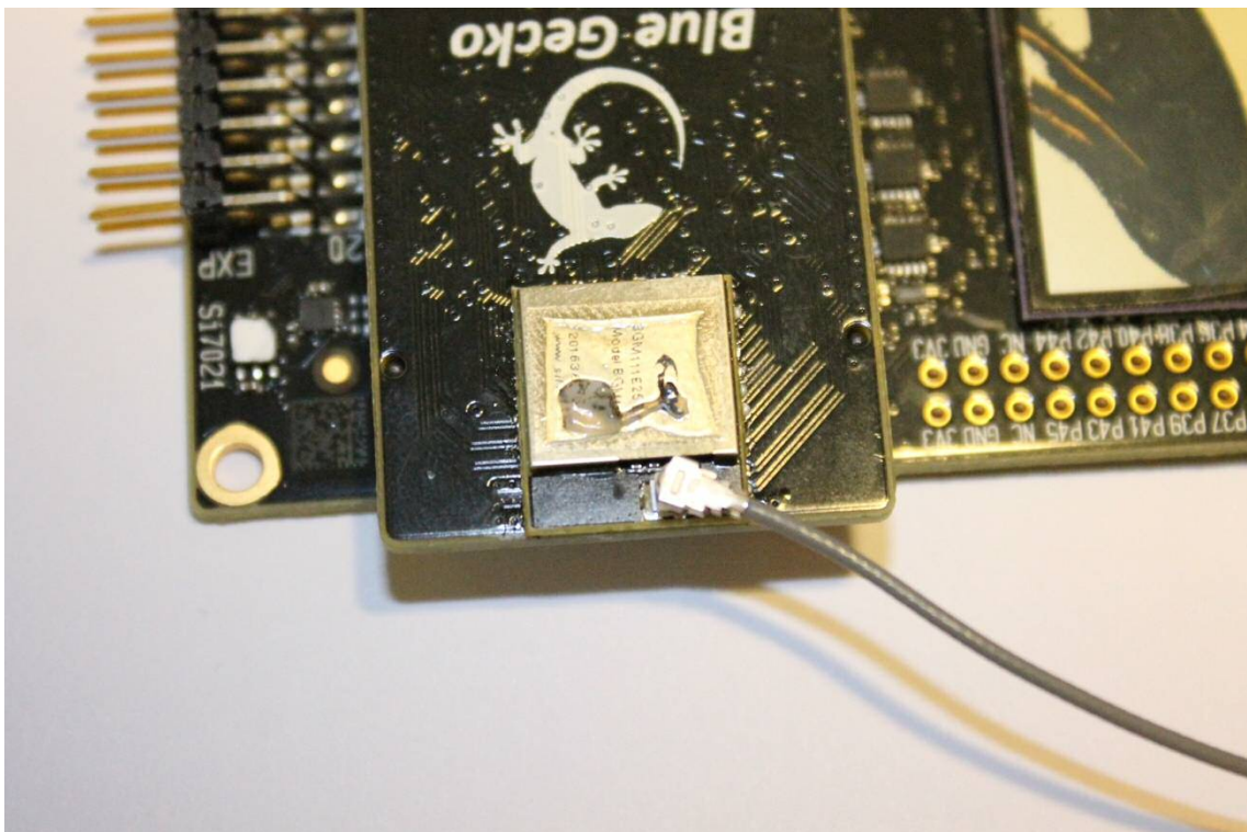
Photograph 6. The EUT
