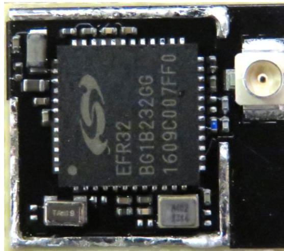
Figure 2: Internal photo of BGM111E
