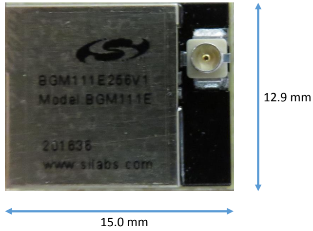
Figure 1: External photo of BGM111E, top view
