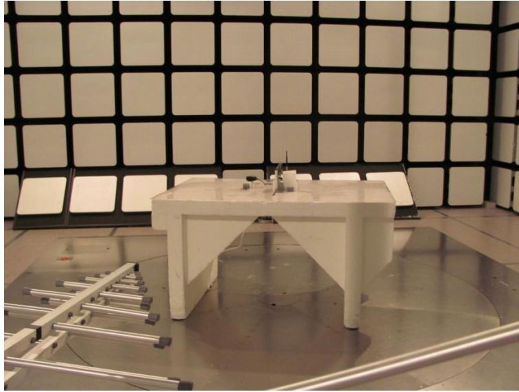
Photograph 1. Radiated emissions 30 - 1000 MHz ext. antenna
