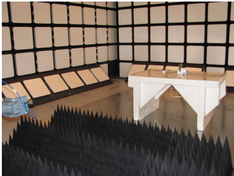
Photograph 6. Radiated emissions 18-26.5 GHz int. antenna
