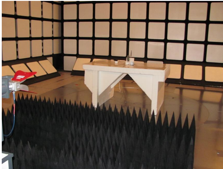
Photograph 3. Radiated emissions 1-18 GHz ext. antenna
