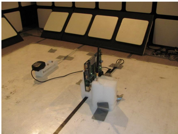
Photograph 8. EUT on table ext. antenna
