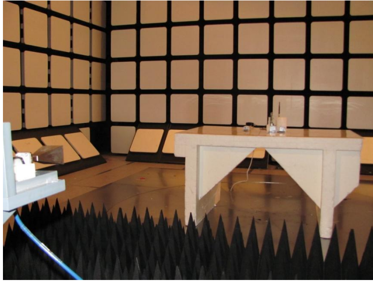
Photograph 5. Radiated emissions 18-26.5 GHz ext. antenna
