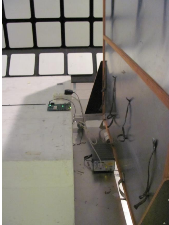
Photograph 9. Conducted Emissions
