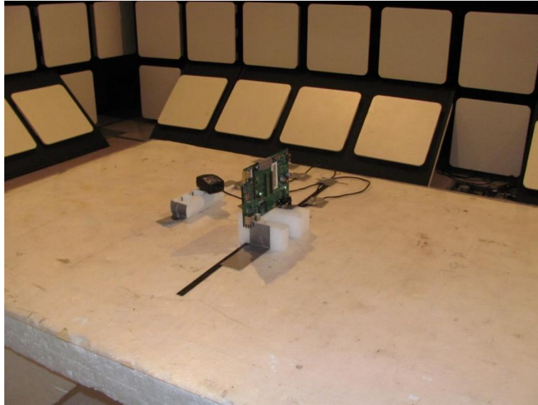
Photograph 7. EUT on table int. antenna
