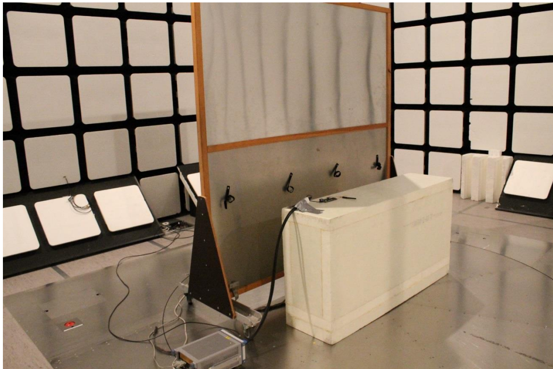
Photograph 10. Conducted Emissions
