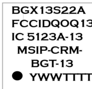
Figure 2: BGX13S22A label
