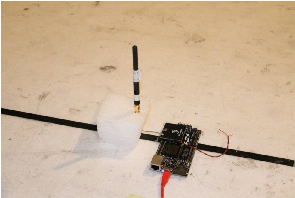
Photograph 4. EUT on table (External antenna)
