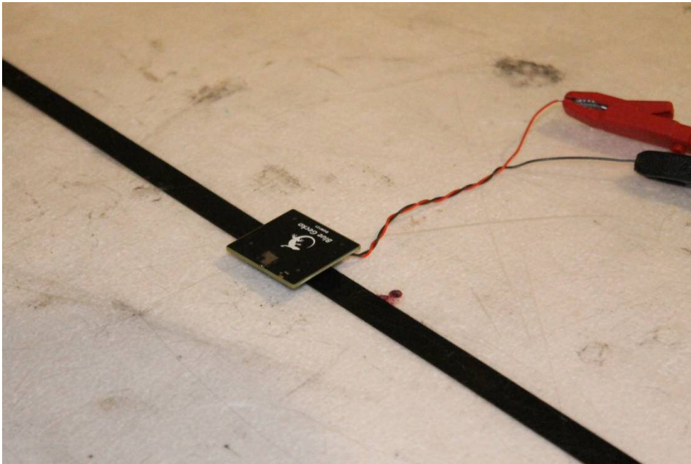
Photograph 5. EUT on table (integral chip antenna)
