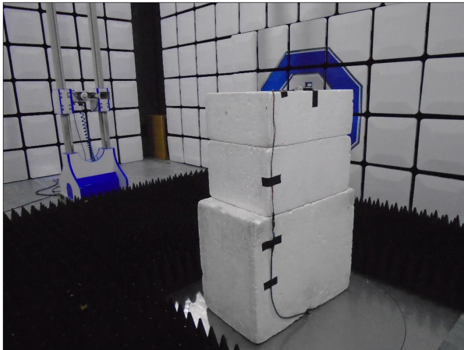
Figure 8 - Test Setup - 8 GHz to 18 GHz - Y
