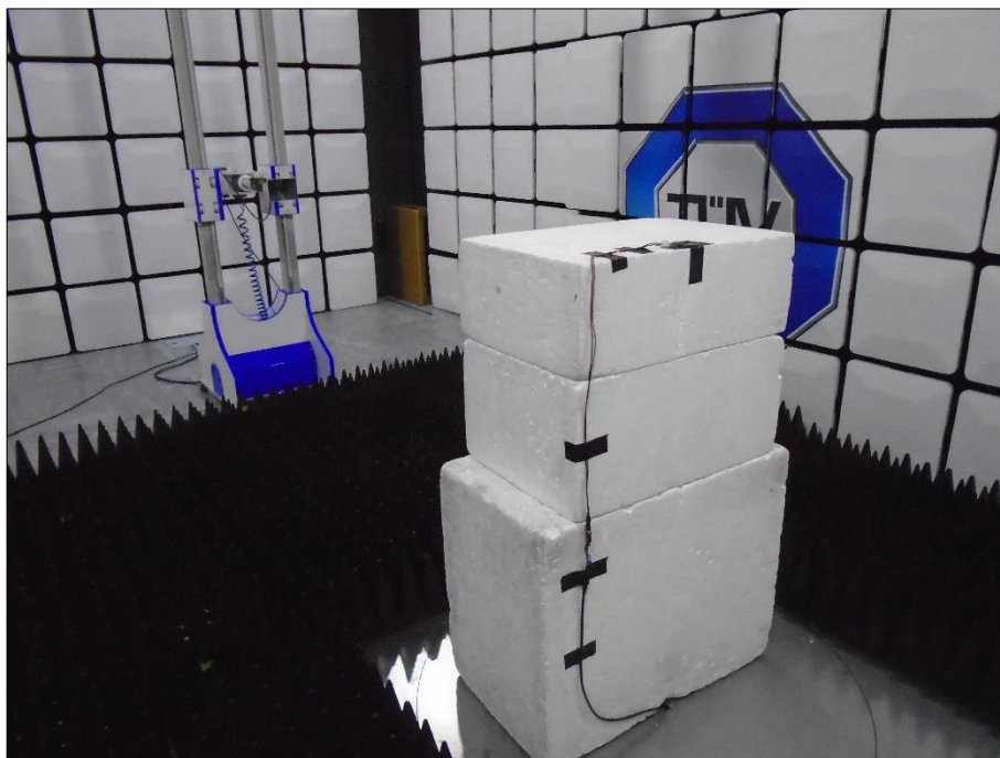
Figure 6 - Test Setup - 1 GHz to 8 GHz - Z
