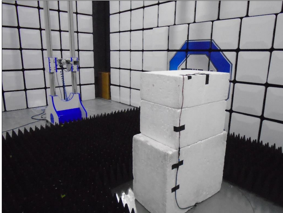
Figure 9 - Test Setup - 8 GHz to 18 GHz - Z
