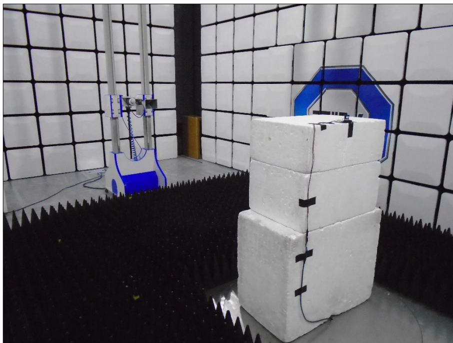
Figure 4 - Test Setup - 1 GHz to 8 GHz - X
