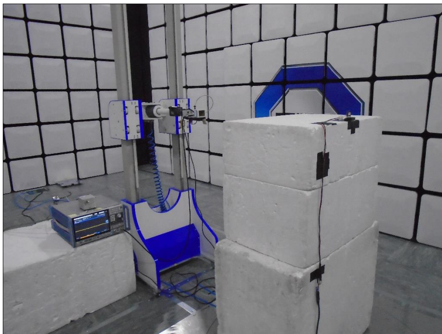
Figure 10 - Test Setup - 18 GHz to 25 GHz - X
