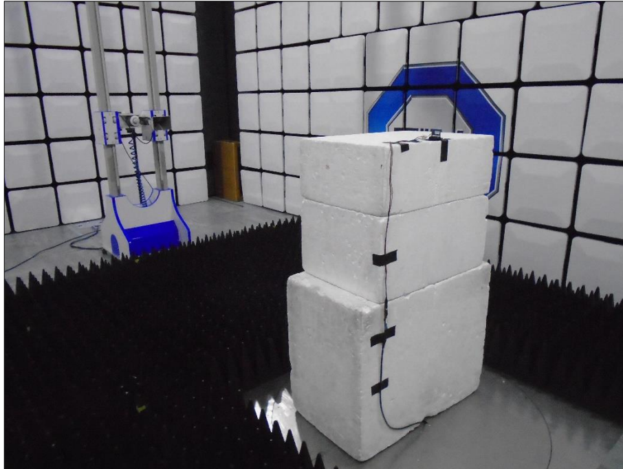
Figure 5 - Test Setup - 1 GHz to 8 GHz - Y
