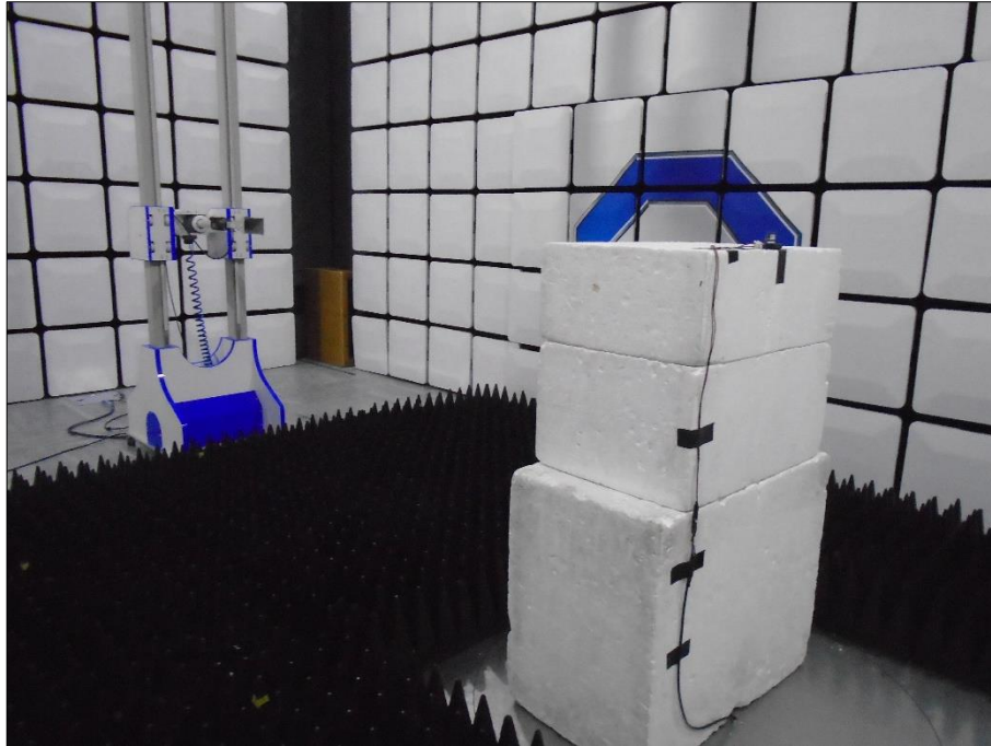
Figure 7 - Test Setup - 8 GHz to 18 GHz - X
