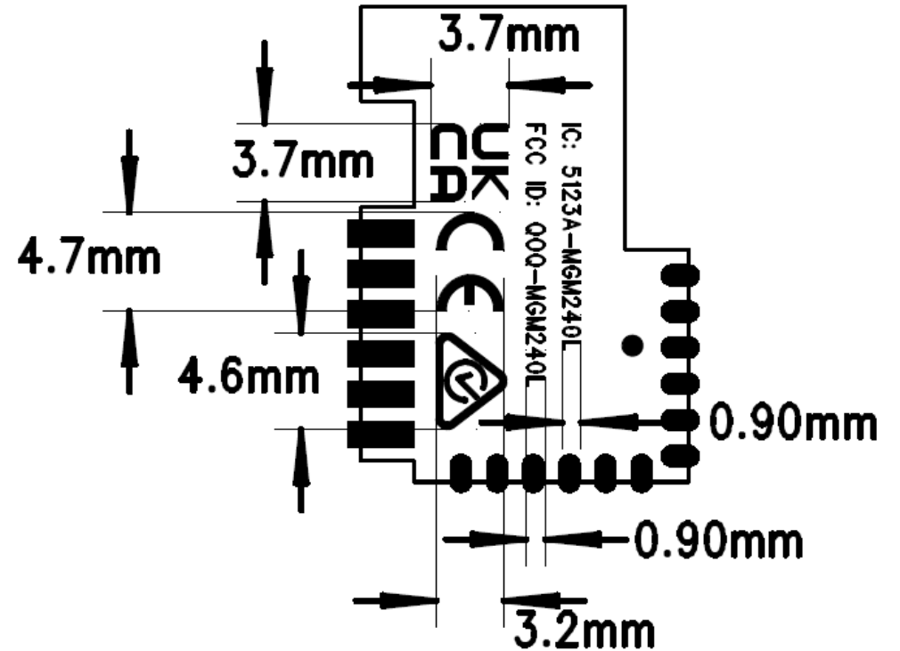
SILK SCREEN
