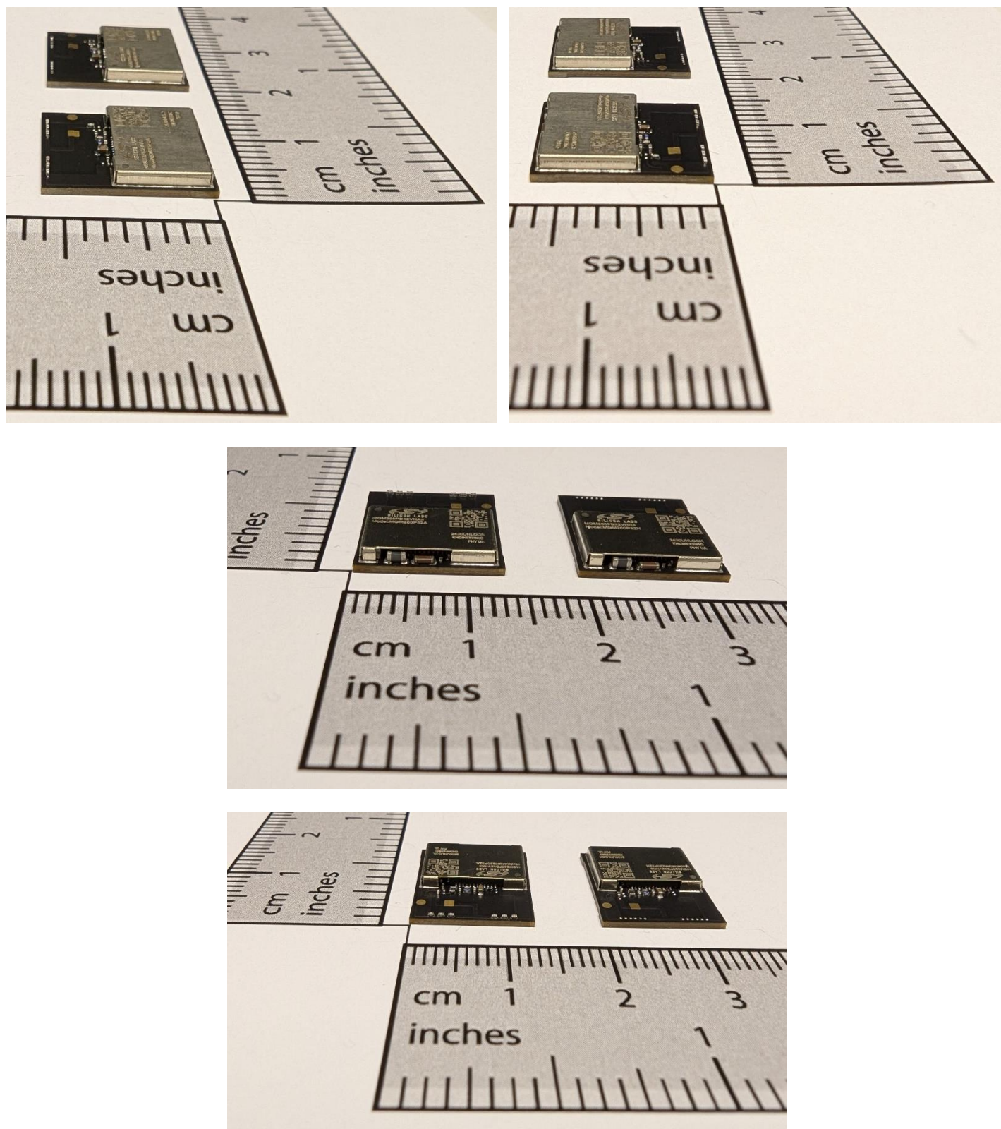
Figure 4: Side Views of the MGM260P32A and MGM260P32N Modules
