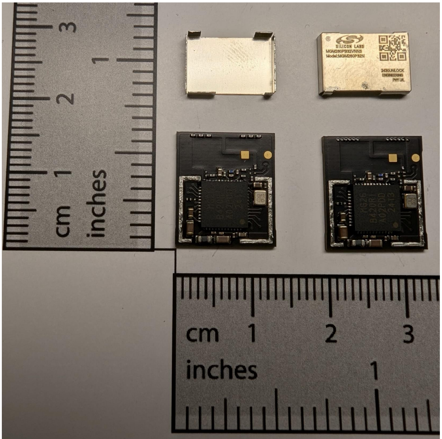
Figure 3: Top/Front Internal View of the MGM260P32A and MGM260P32N Modules
