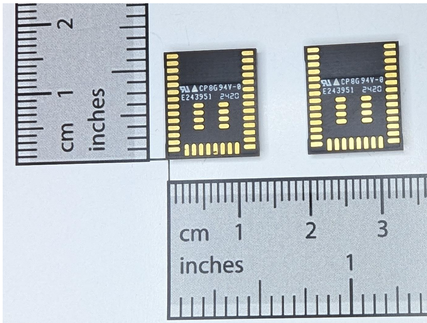
Figure 2: Bottom/Rear External View of the MGM260P32A and MGM260P32N Modules
