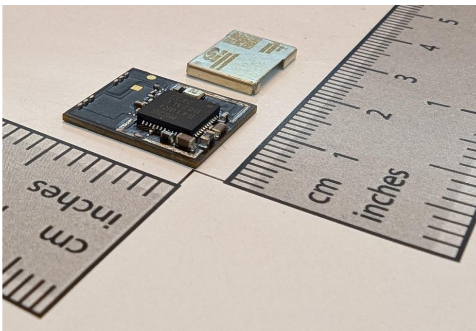
Figure 4: Internal Side View of the MGM260P22A Module
