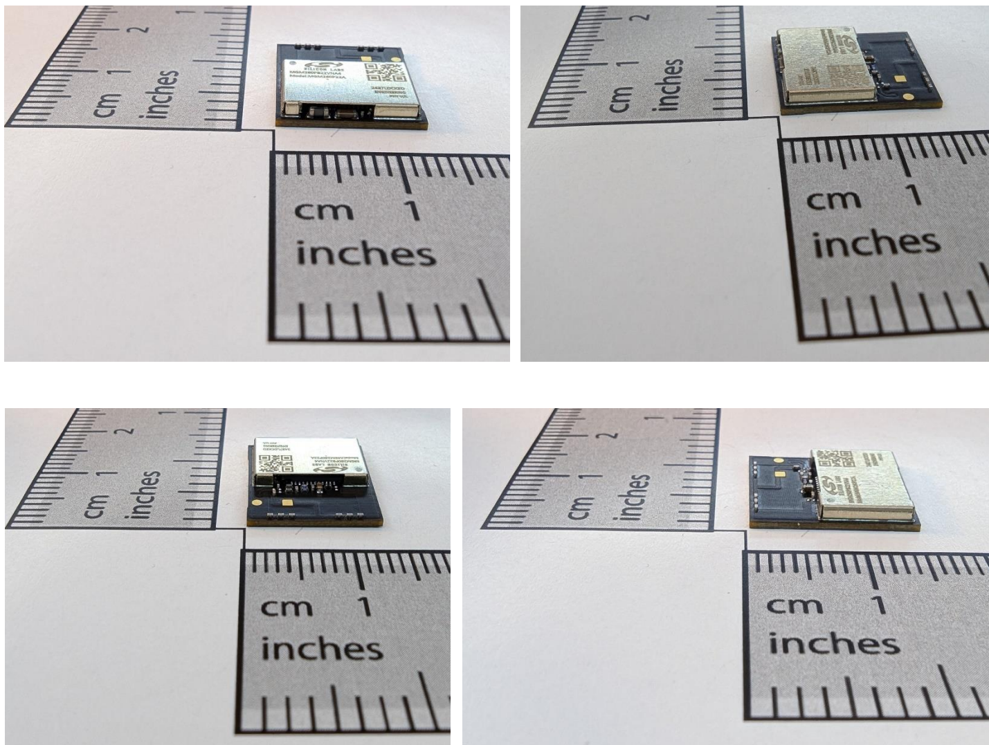
Figure 5: Side Views of the MGM260P22A Module
