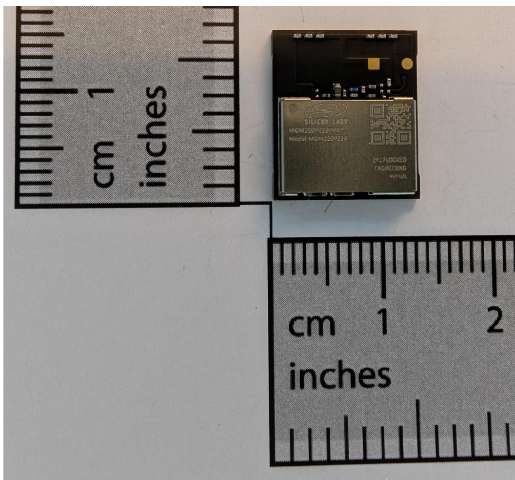
Figure 1: Top/Front External View of the MGM260P22A (low-power variant of the family of xGM260Px modules, with integral antenna)
