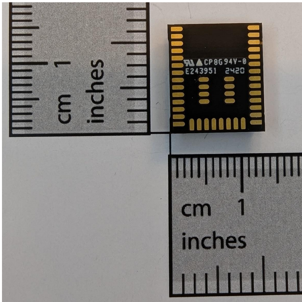
Figure 2: Bottom/Rear External View of the MGM260P22A Module
