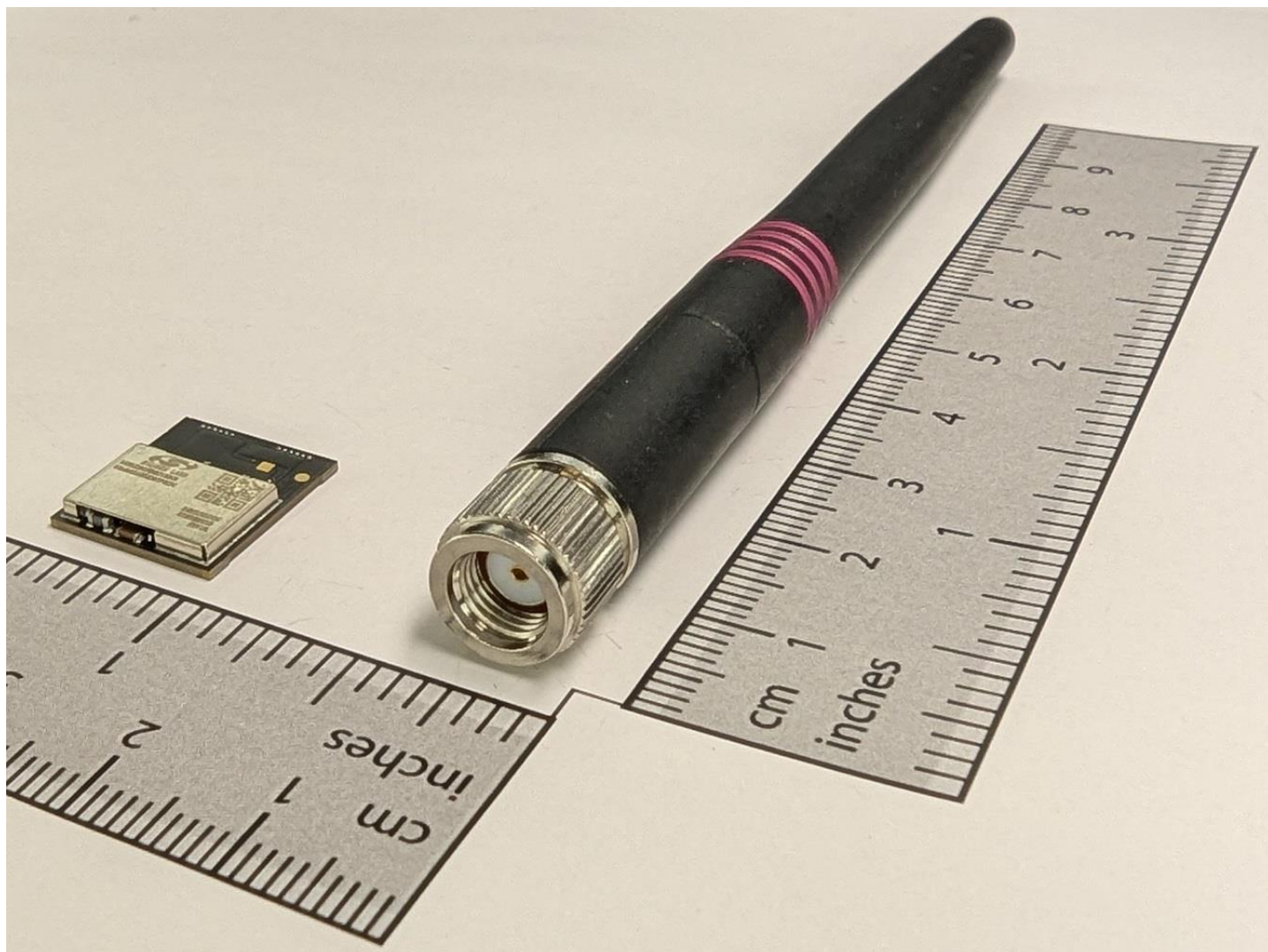
Figure 3: Oblique Full View of the Reference External Antenna, next to the MGM260P32N Module
