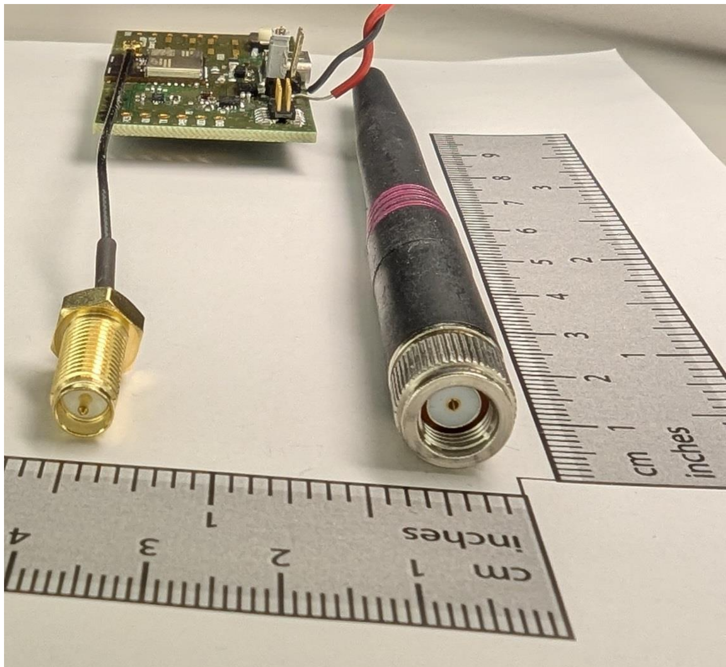
Figure 6: Detail of the SMA Connectors of the Reference External Antenna, and of the SMA+U.FL Terminated Thin Coax cable
