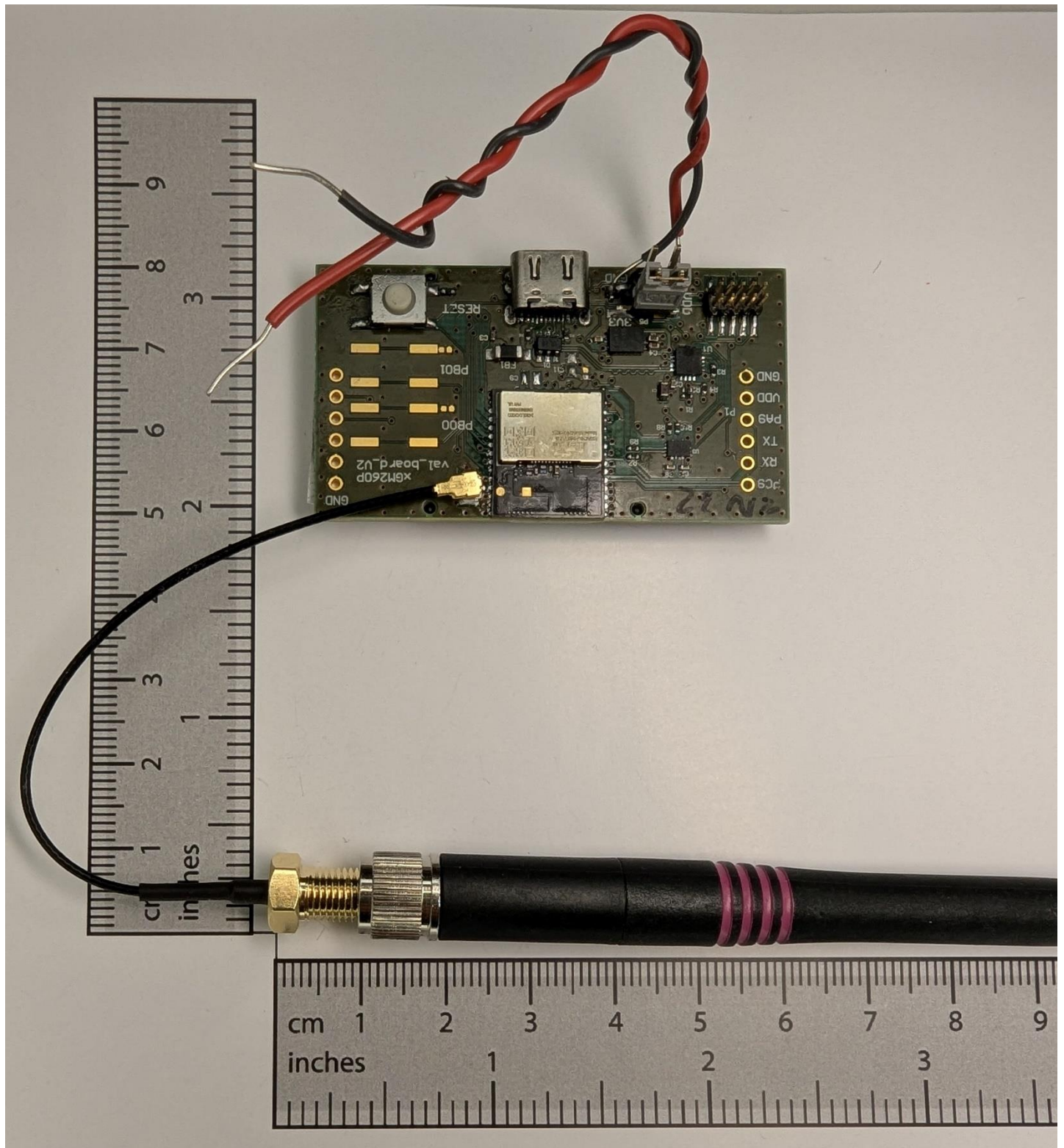
Figure 7: View of the Reference External Antenna Connected to the MGM260P32N module via the Thin Coax Cable and the Related Antenna Connectors
