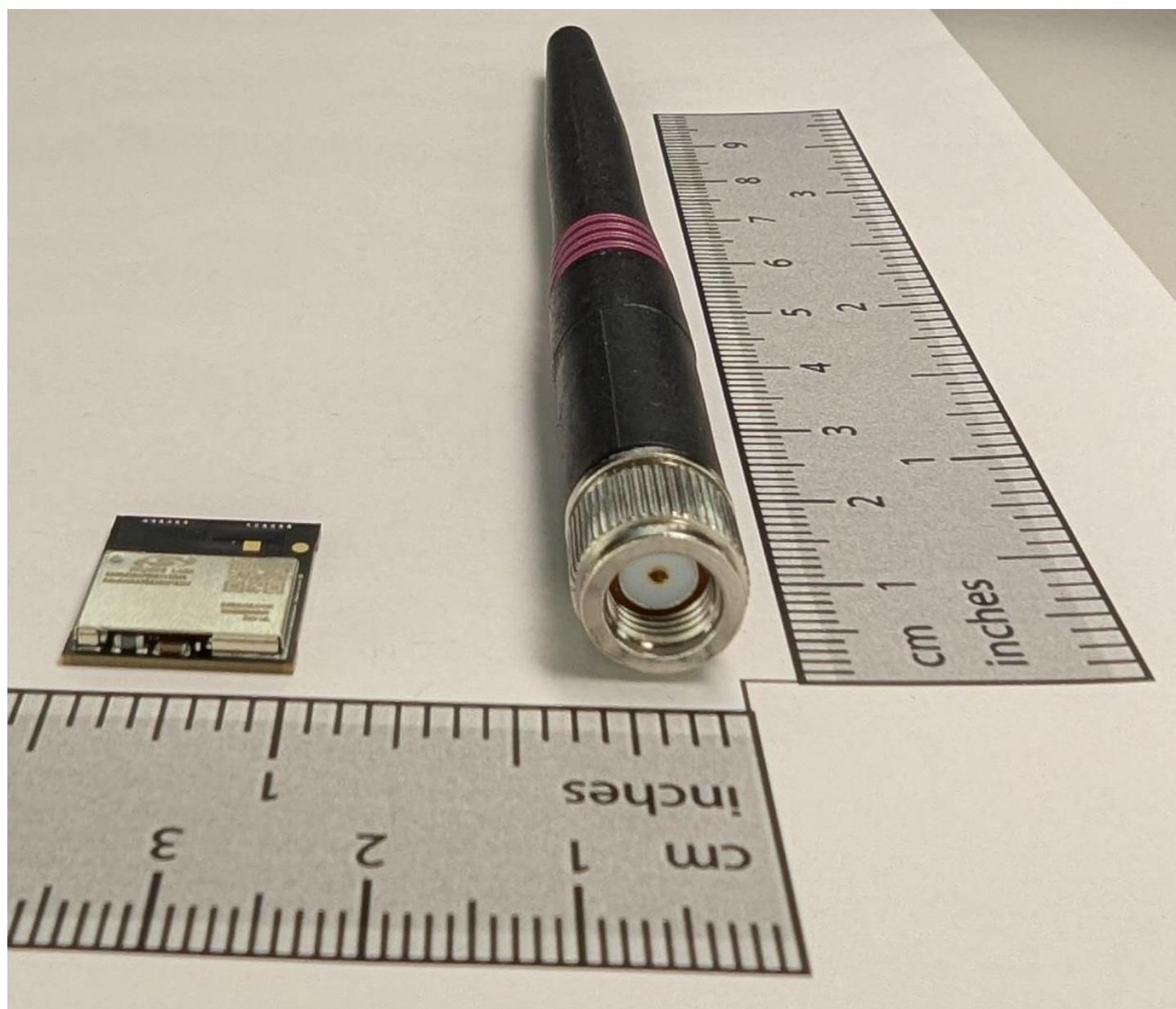
Figure 2: Vertical Full View of the Reference External Antenna, next to the MGM260P32N Module
