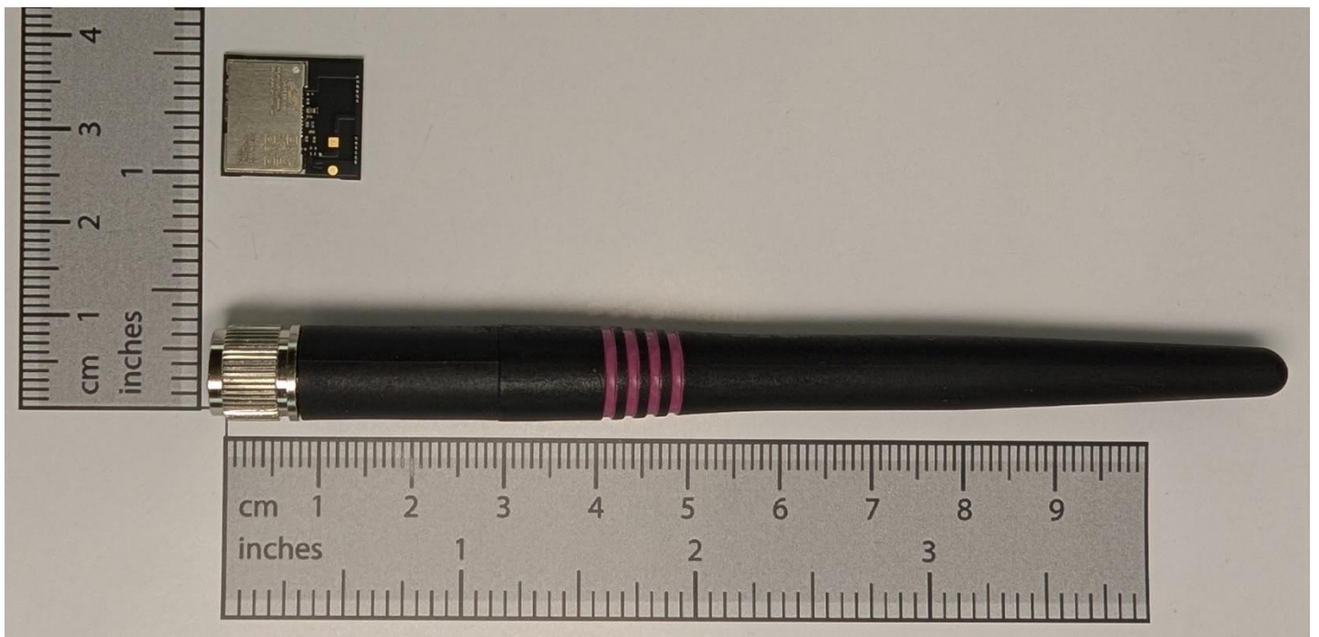
Figure 1: Horizontal Full View of the Reference External Antenna, next to the MGM260P32N Module – Antenna is the ANT-2.4-CW-CT-RPS by TE Connectivity
