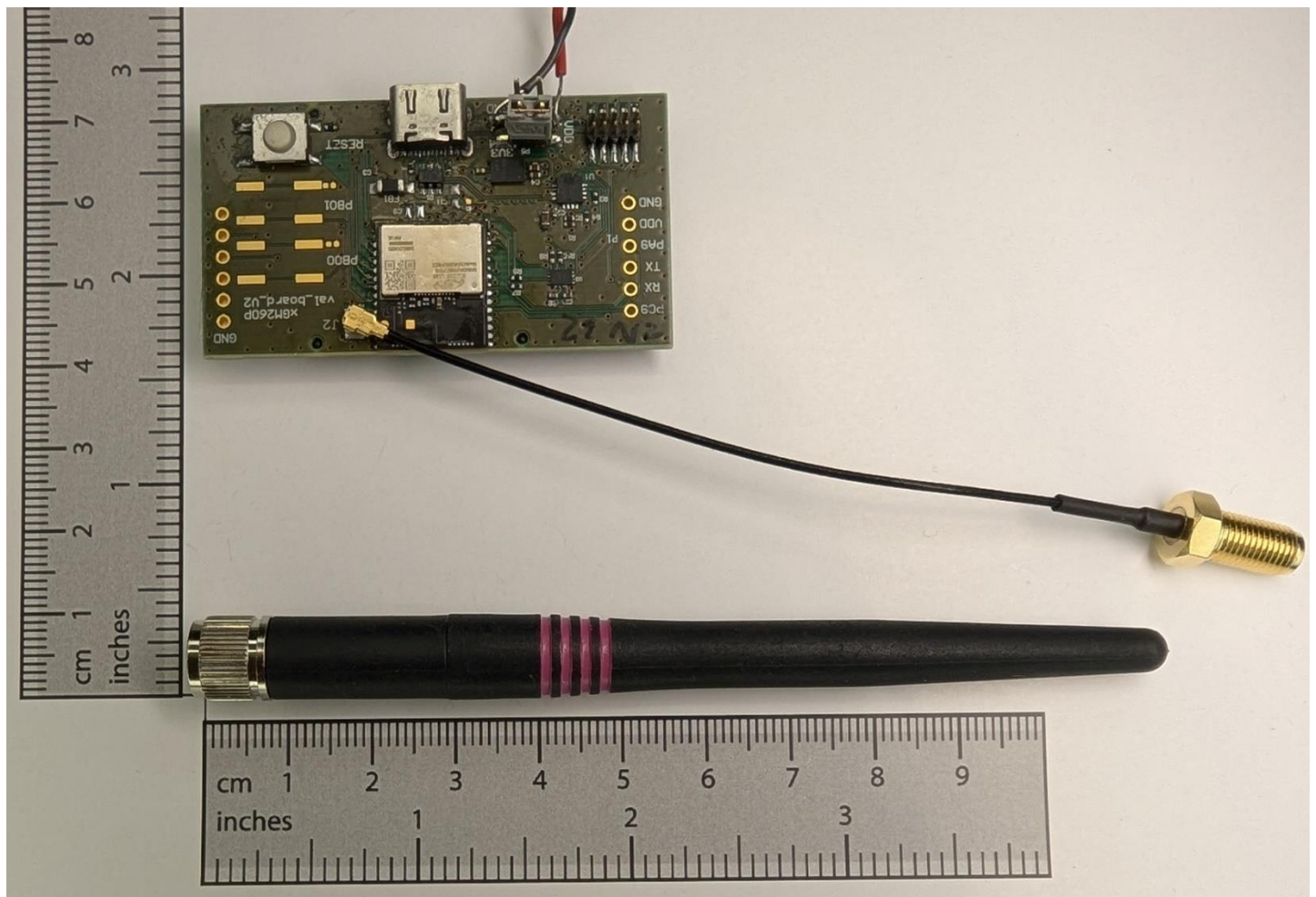
Figure 5: Full View of the Reference External Antenna, next to the Certification host board carrying the MGM260P32N Module
