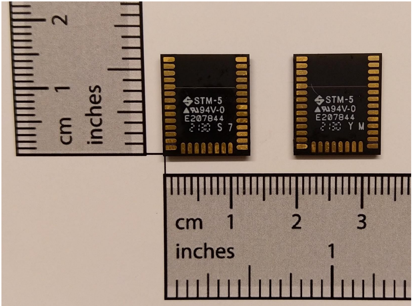
Figure 4: Bottom/Rear External View of the MGM240P32A Modules
