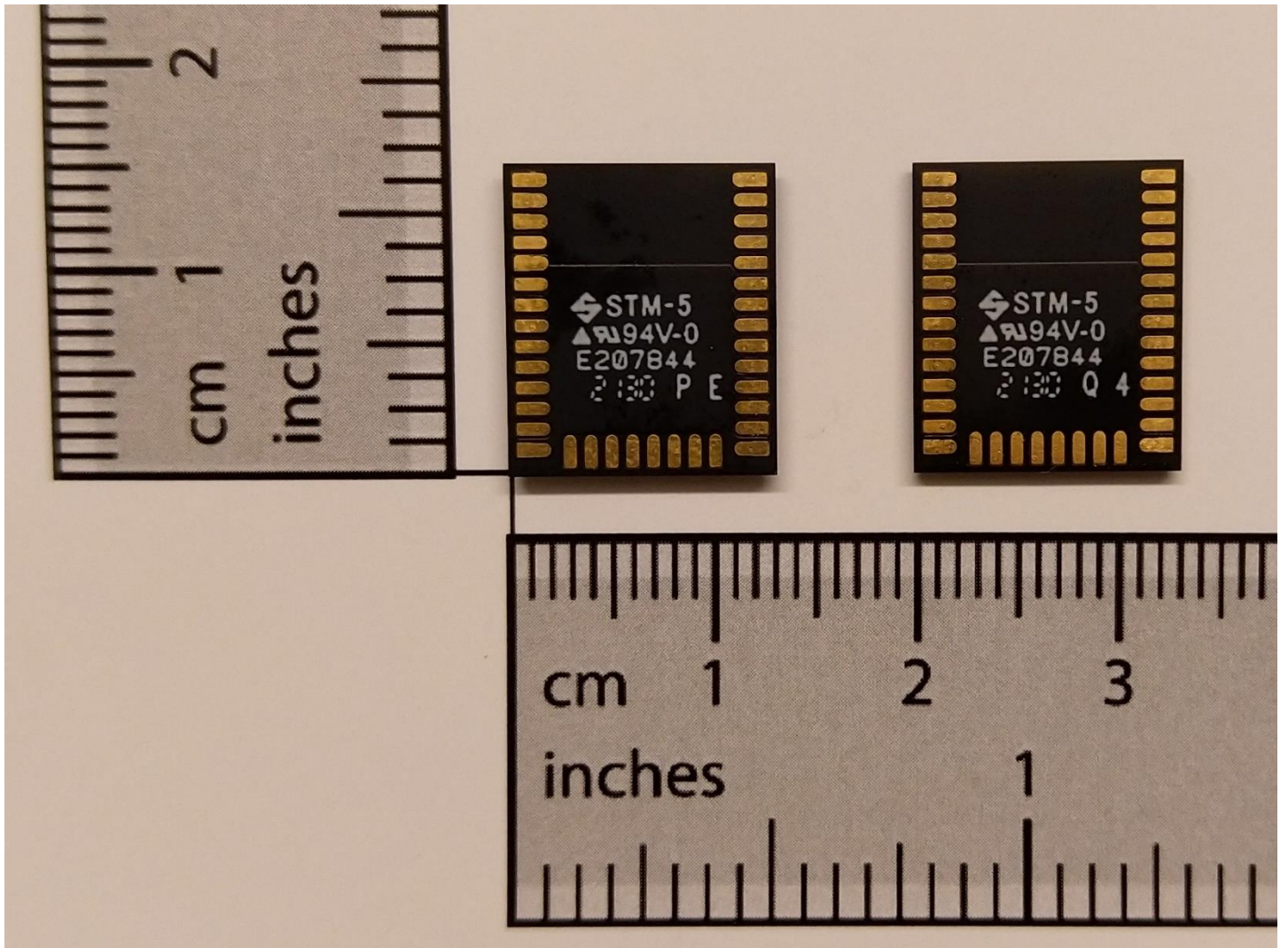
Figure 2: Bottom/Rear External View of the MGM240P22A Modules
