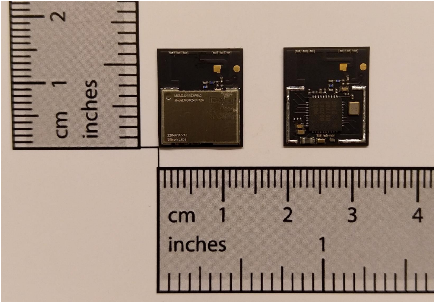
Figure 3: Top/Front External and Internal View of the MGM240P32A Modules
