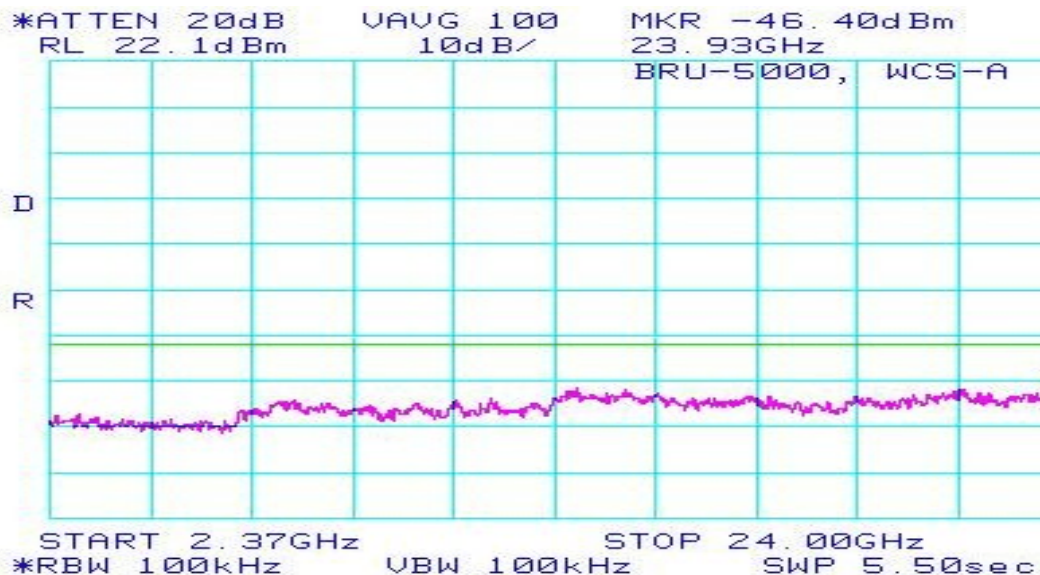
Plot #10: WCSA Spurious Emission 2.37 - 24 GHz
