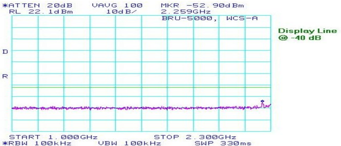
Plot #6: WSA Spurious Emission 1 - 2.3 GHz
