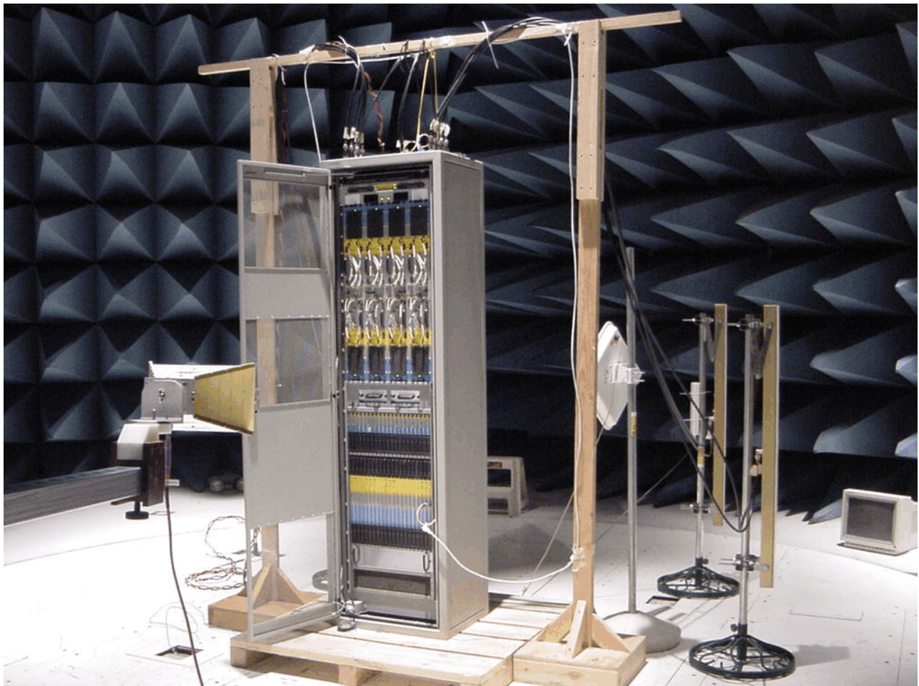
Photograph 5. Radiated Emissions Test Setup Photo (1 - 24 GHz)
