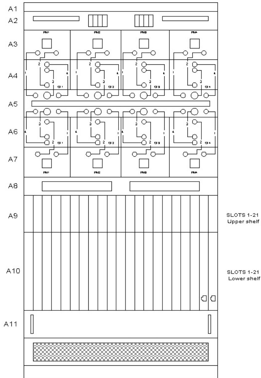
Figure 2. Port Identification
