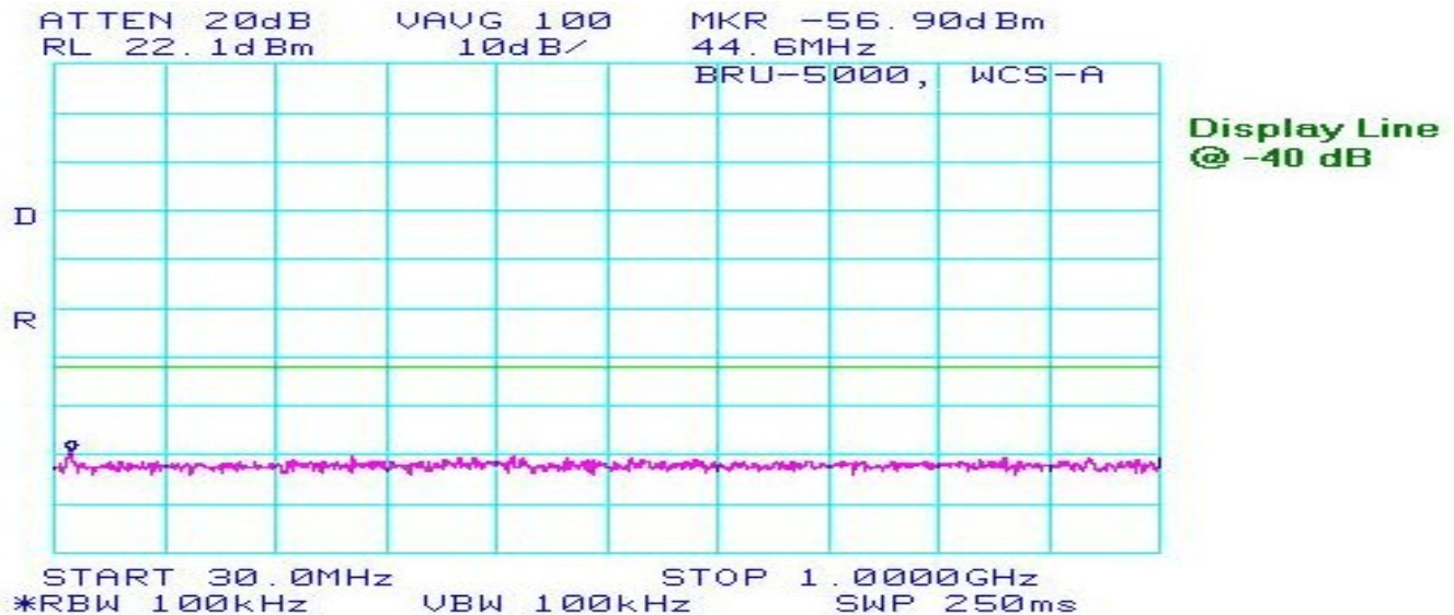
Plot #5: WSA Spurious Emission 30 MHz - 1 GHz
