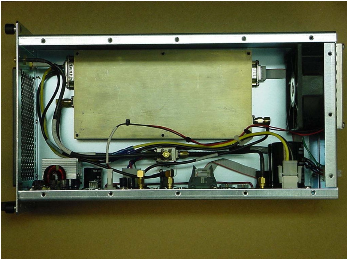
Photograph 18. PM without Heat Sink
