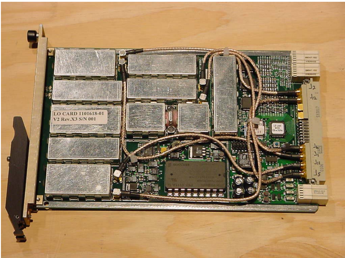
Photograph 8. LO Top
