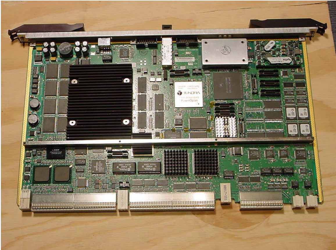
Photograph 2. DS3 and OC3 NPC Top
