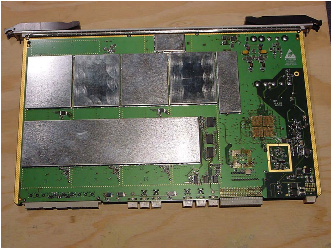
Photograph 27. XCVR Bottom
