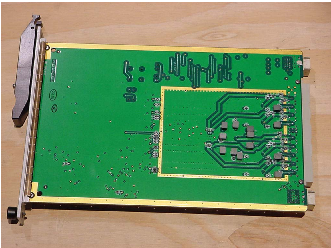
Photograph 24. RFSW Bottom
