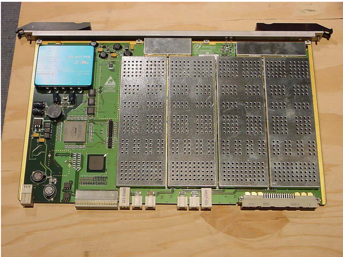
Photograph 26. XCVR Top
