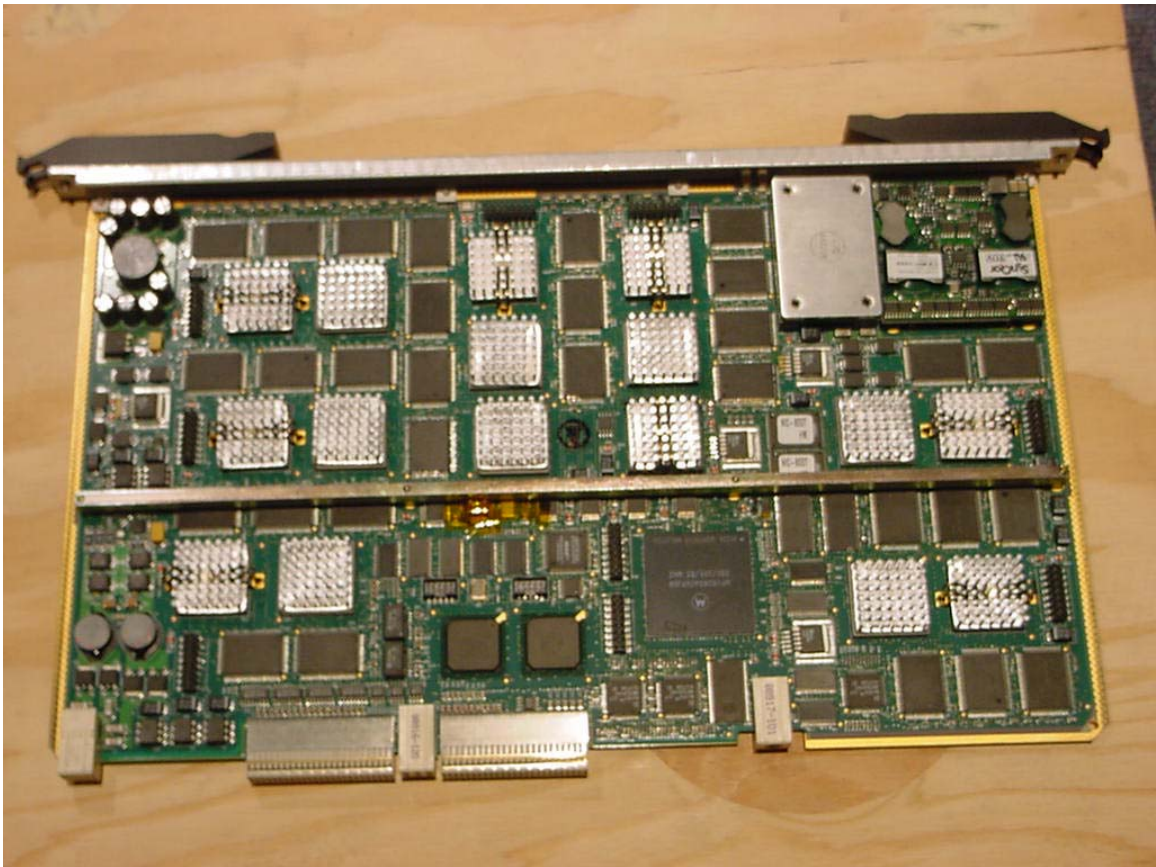
Photograph 11. MBP Top
