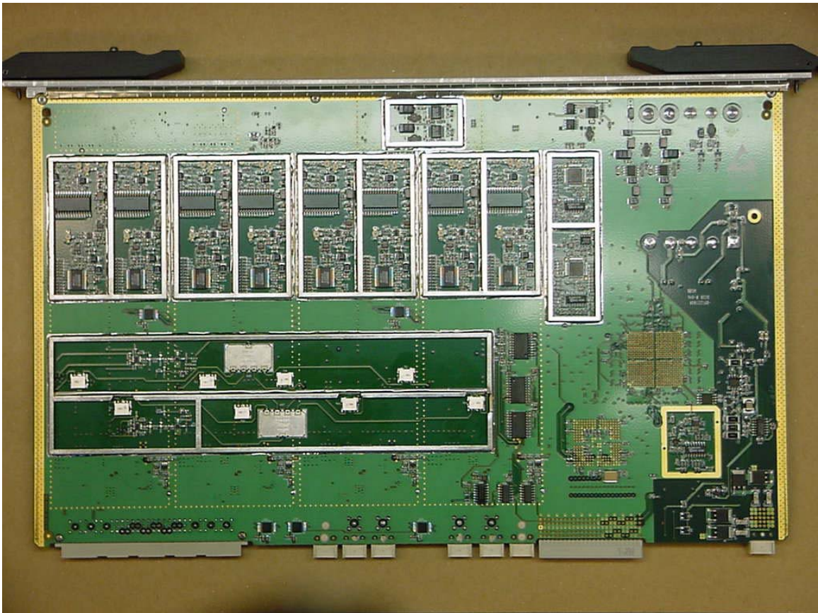
Photograph 29. XCVR Bottom without Shield Cover
