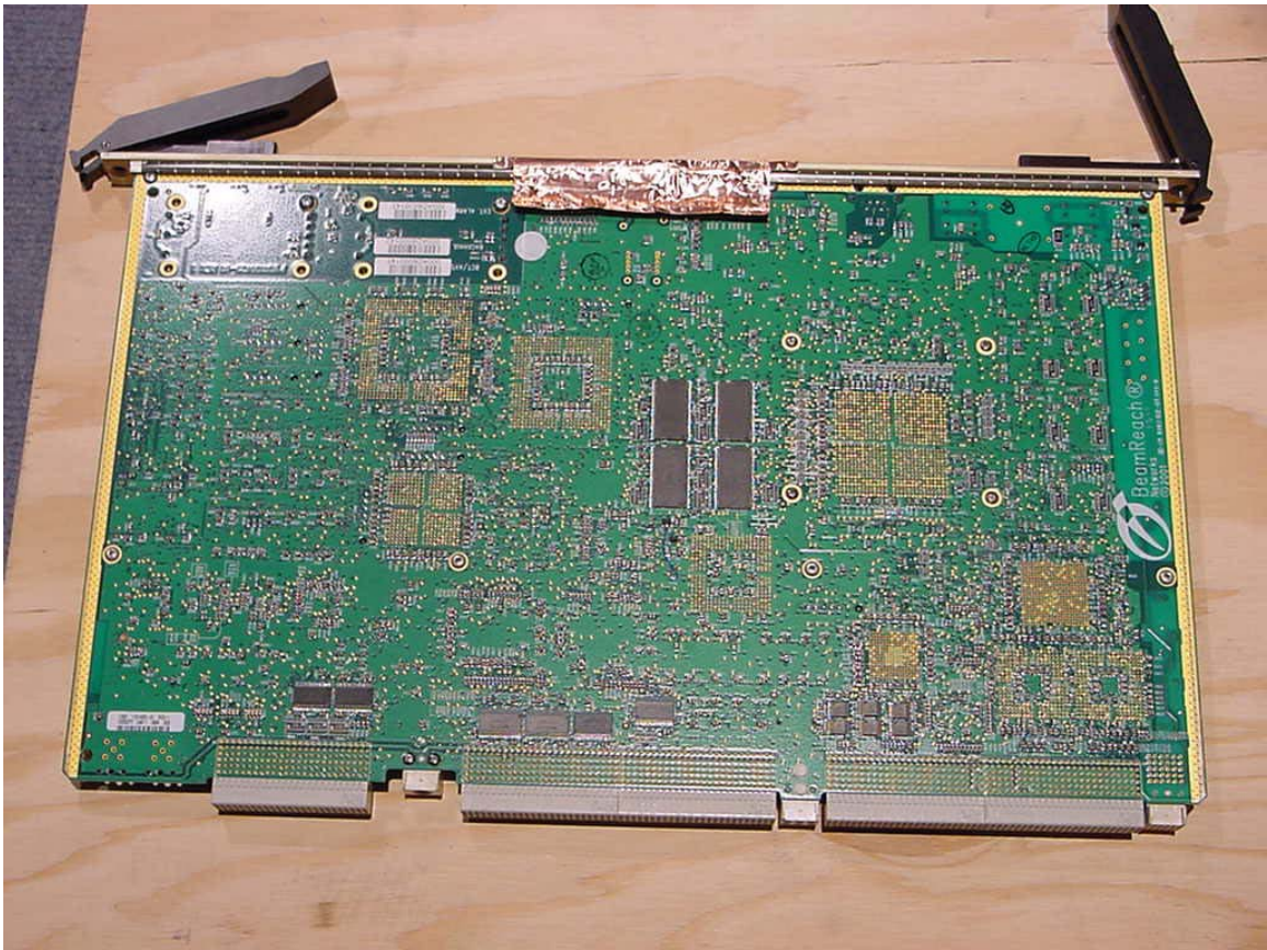
Photograph 7. Fast Ethernet NPC Bottom
