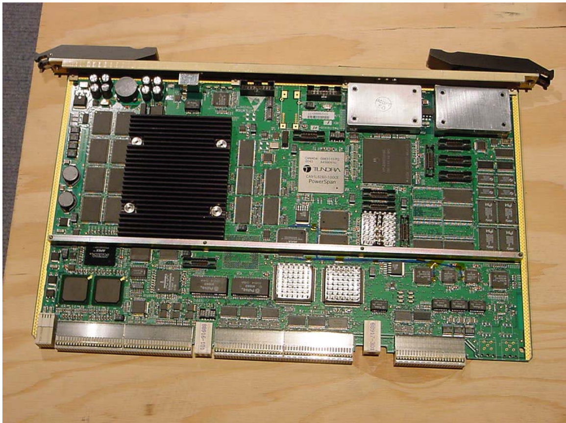
Photograph 6. Fast Ethernet NPC Top
