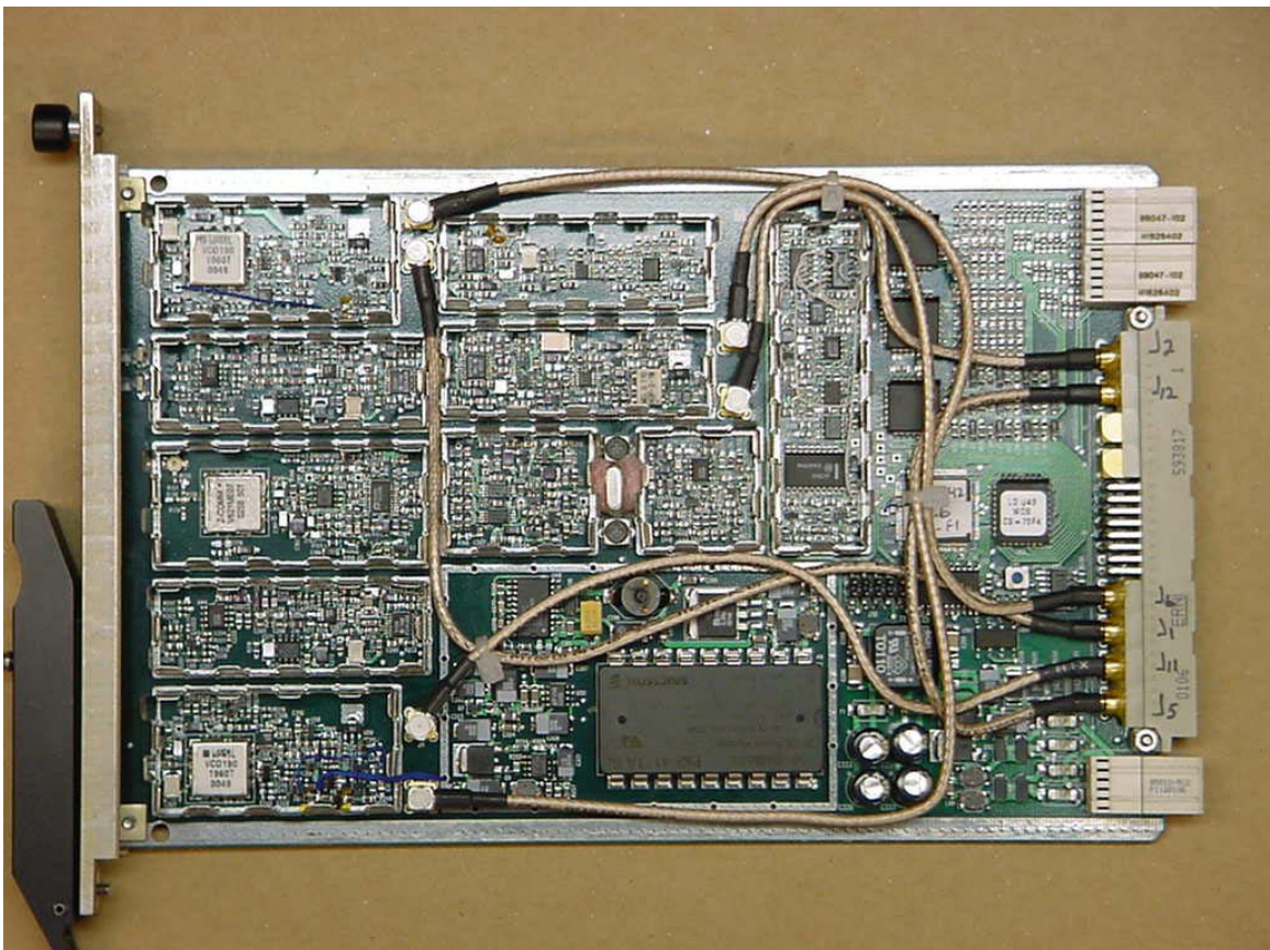
Photograph 10. LO Top without Shield Cover
