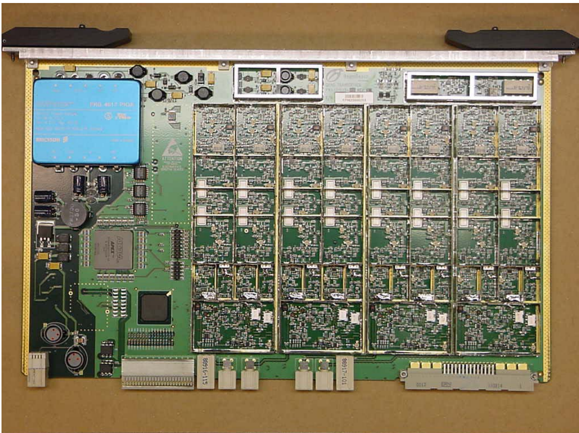
Photograph 28. XCVR Top without Shield Cover
