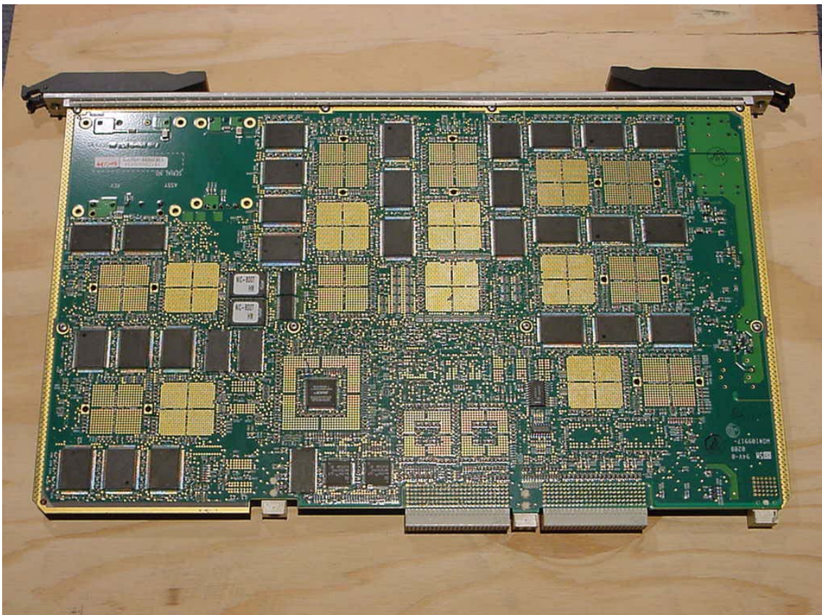
Photograph 12. MBP Bottom
