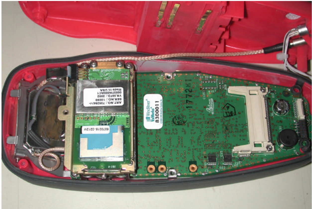
Photo 2 Detail View – Unit opened – bluetooth module shown
