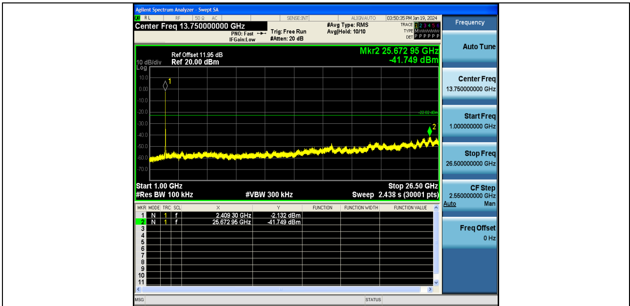
11N20SISO-Ant1-2412-1000~26500-PASS
