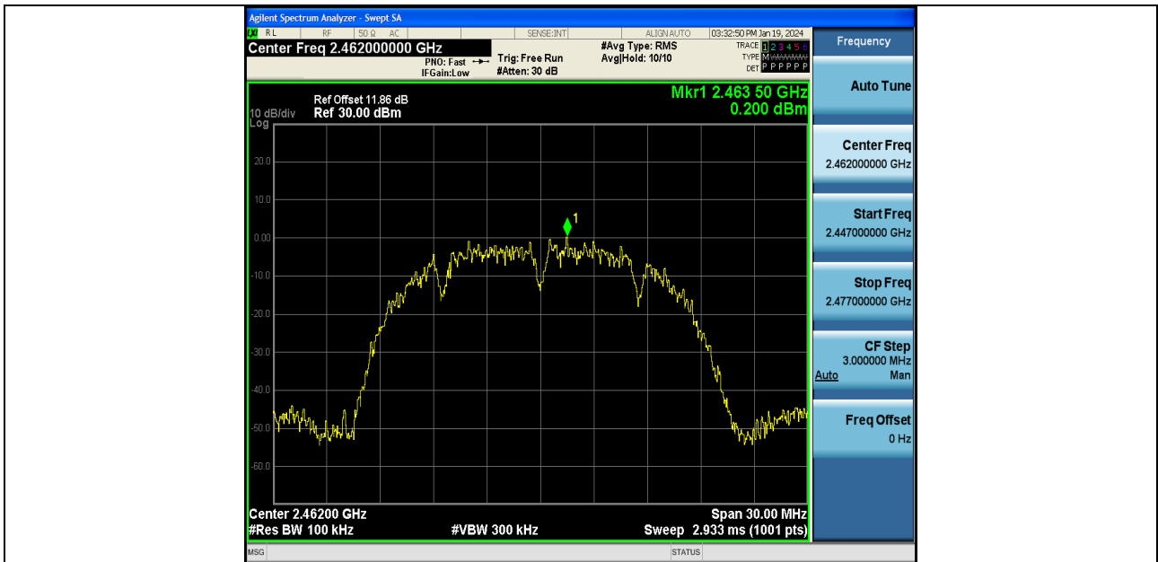
11B-Ant1-2462-0~Reference-PASS
