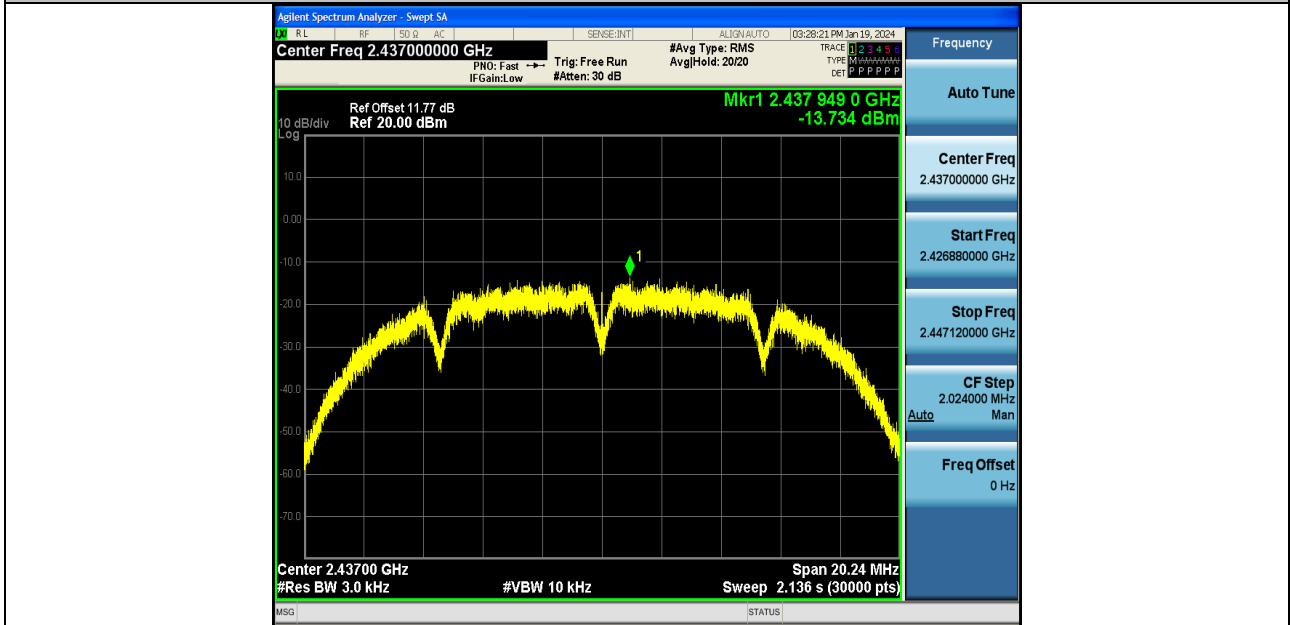
11B-Ant1-2437-PASS
