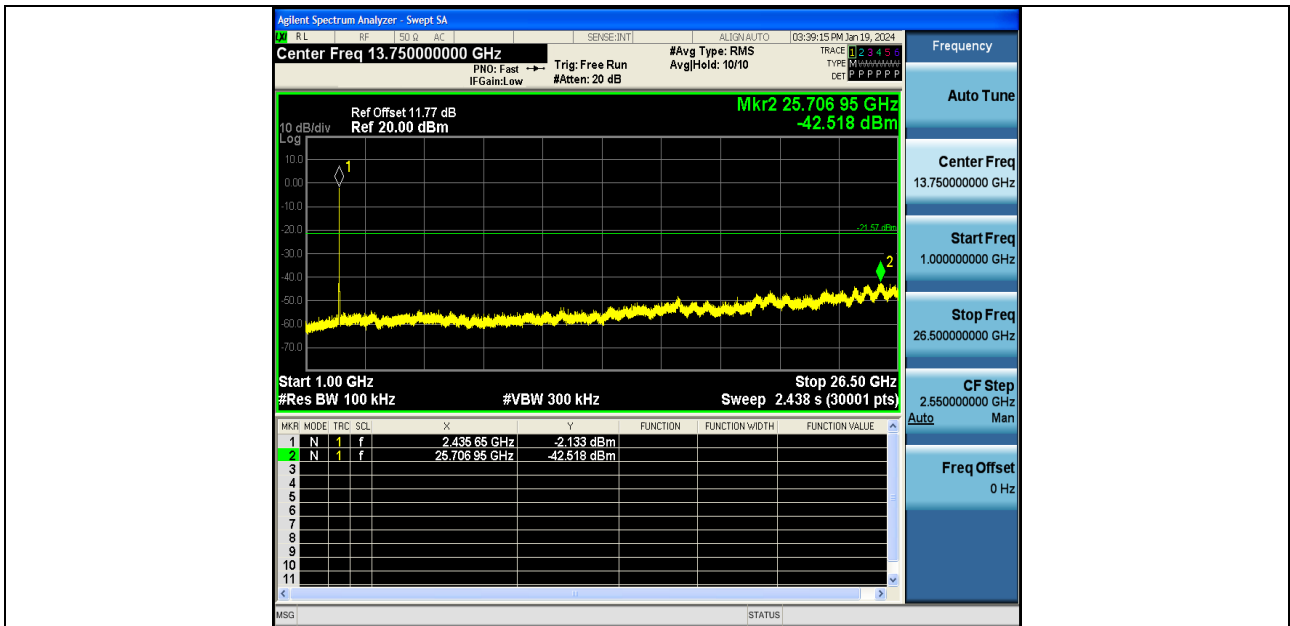
11G-Ant1-2437-1000~26500-PASS
