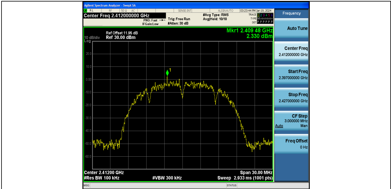
11B-Ant1-2412-0~Reference-PASS
