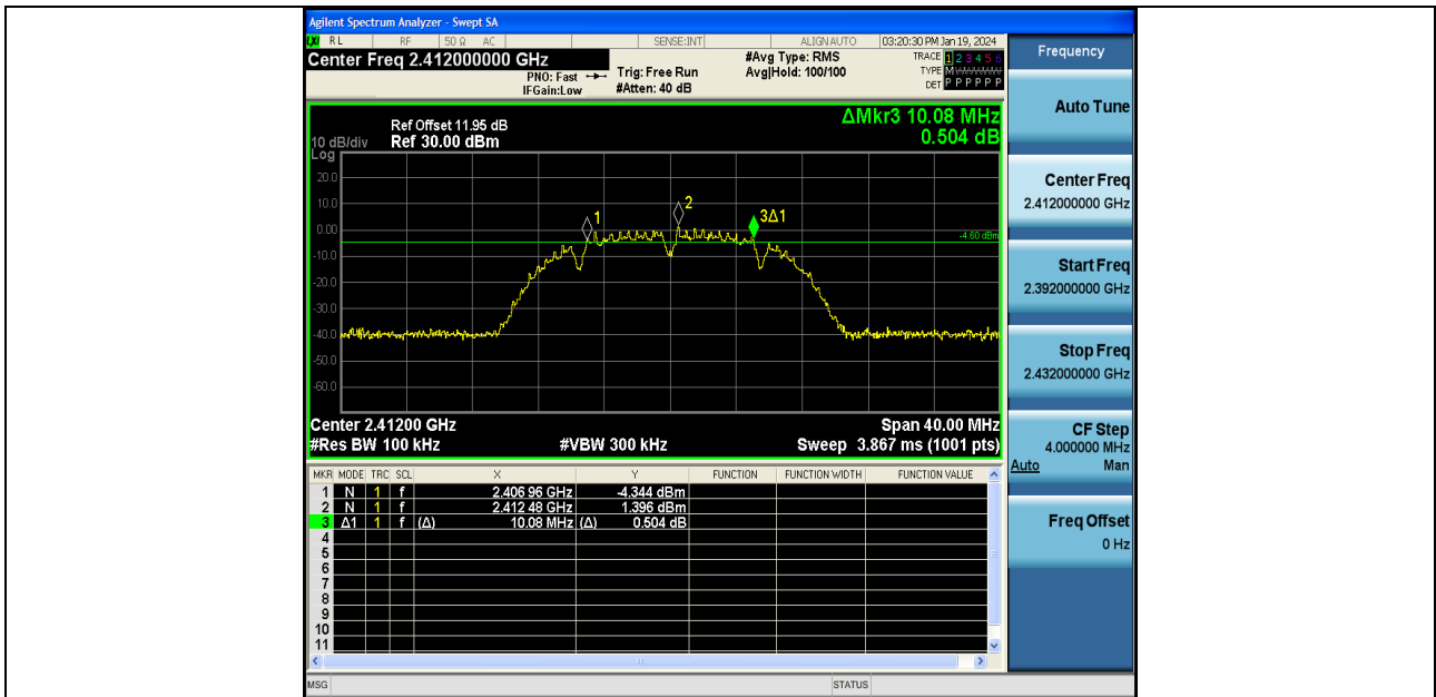
11B-Ant1-2412-PASS
