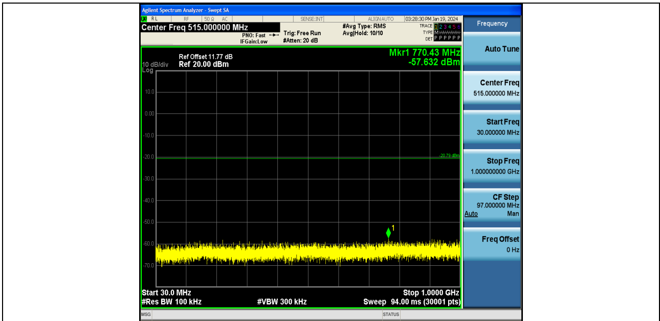
11B-Ant1-2437-30~1000-PASS
