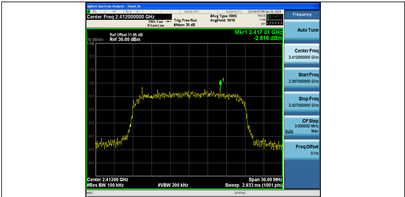
11N20SISO-Ant1-2412-0~Reference-PASS
