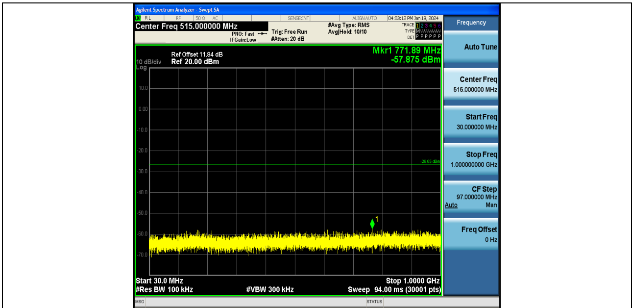
11N40SISO-Ant1-2422-30~1000-PASS
