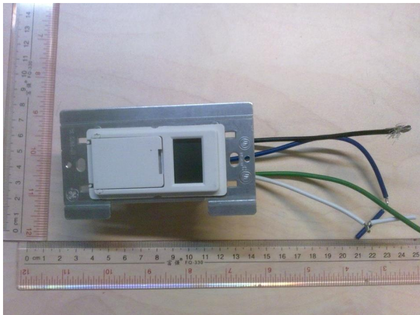
(8) EUT External Photo-Rx Unit
