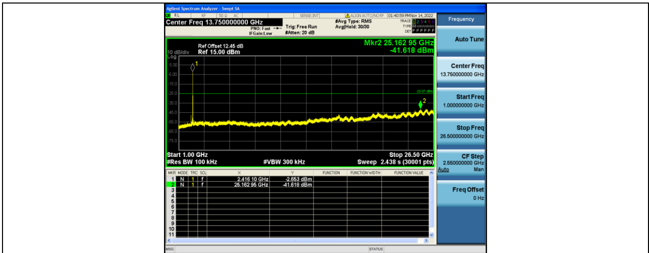
11G-Ant1-2437-0~Reference--6.75
