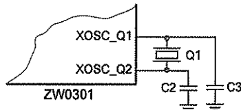
Figure 5: External crystal connections
