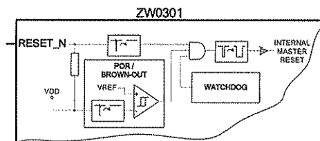
Figure 6: Reset interface
