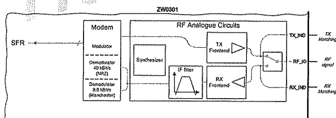
Figure 2: RF transceiver architecture
