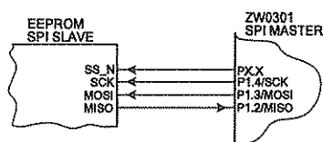
Figure 20: Typical interface to EEPROM
