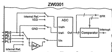
Figure 18: ADC block
