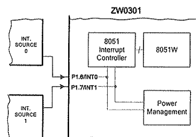
Figure 10: External interrupts
