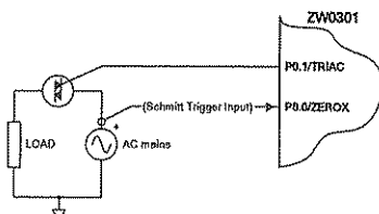
Figure 11: Simplified triac control application
