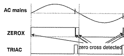
Figure 13: Zero cross signal noise
