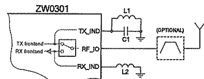
Figure 7: RF interface in typical application
