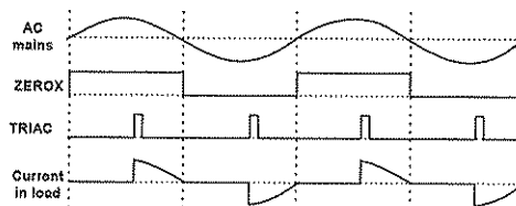
Figure 12: Typical triac waveforms
