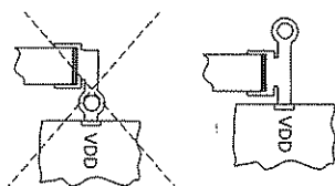
Figure 22: Optimal placement of via
