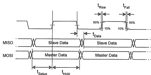
Figure 25: SPI timing
