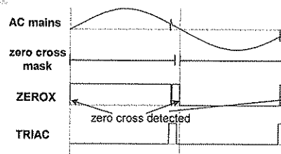
Figure 14: Zero cross signal noise mask
