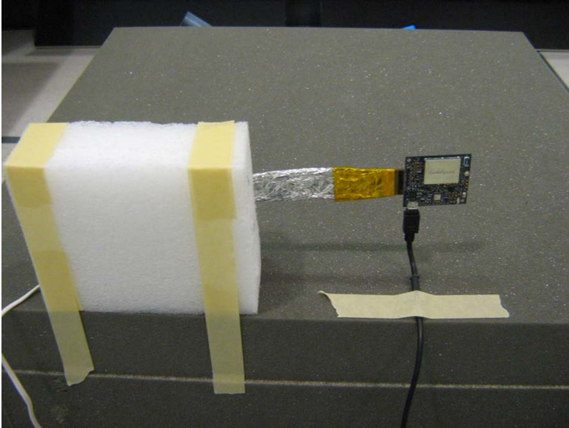
Figure 9: Radiated Emission Setup with EUT on Z-Axis
