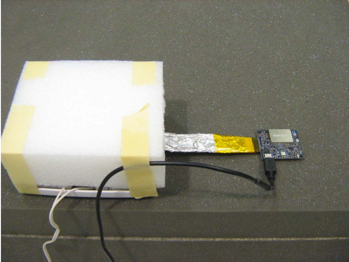
Figure 7: Radiated Emission Setup with EUT on X-Axis
