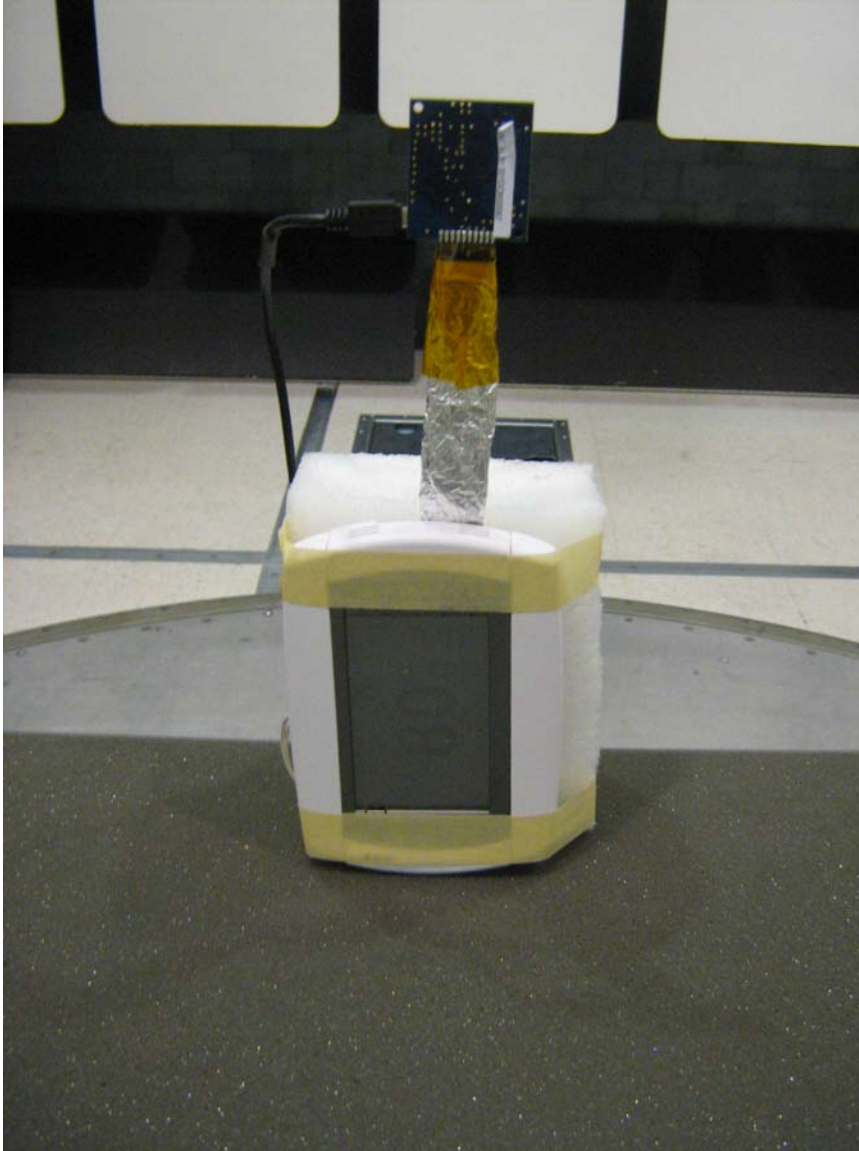
Figure 8: Radiated Emission Setup with EUT on Y-Axis
