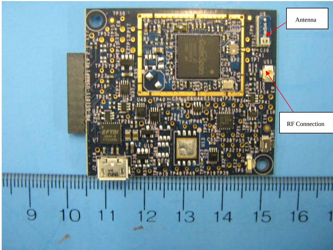
Figure 1: Internal Photo of USNAP WiFi Module without RF Shielded Housing (Front Side)
