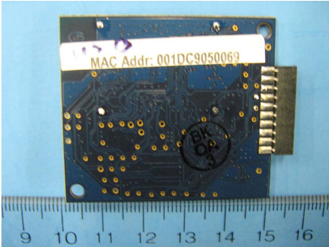
Figure 2: Internal Photo of USNAP WiFi Module without RF Shielded Housing (Rear Side)
