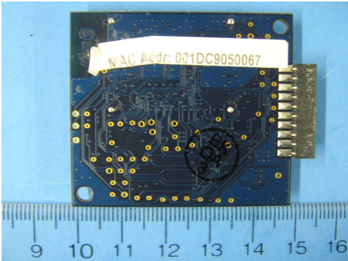
Figure 2: External Photo of USNAP WiFi Module (Soldered Side)
