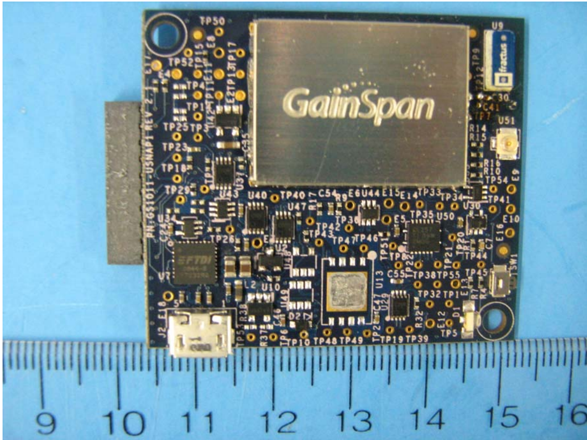
Figure 1: External Photo of USNAP WiFi Module (Component Side)
