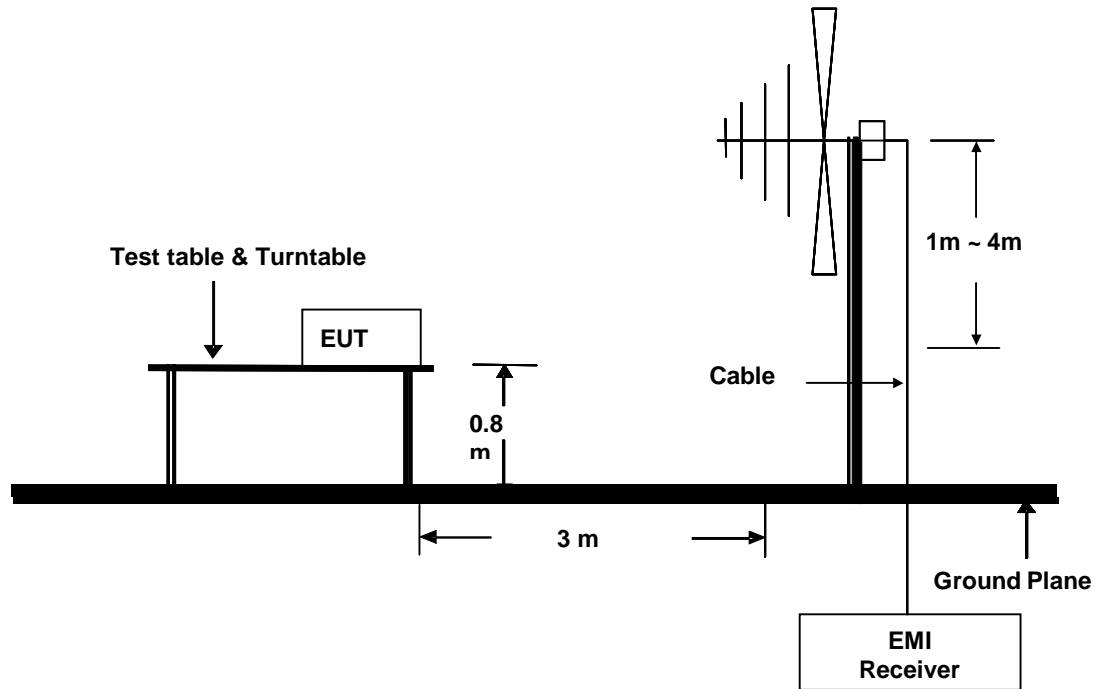
Figure 1. 30MHz to 1GHz radiated emissions test configuration
