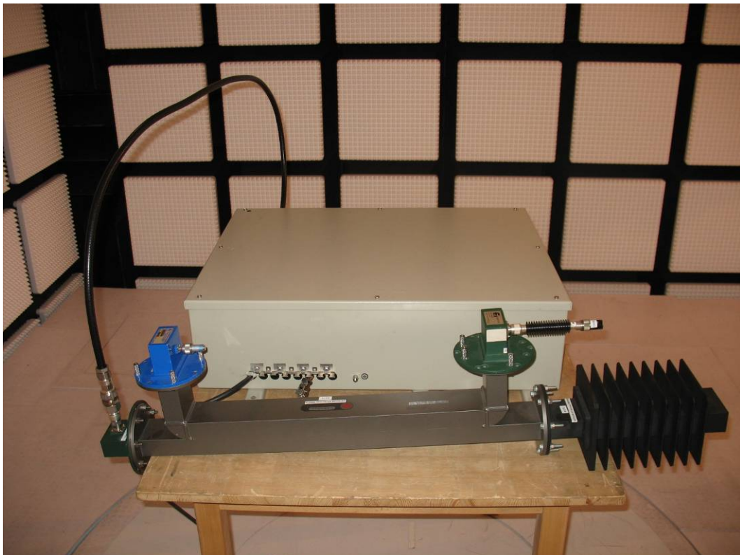
Photo No. 4: radiated spurious emissions up to 12 GHz
