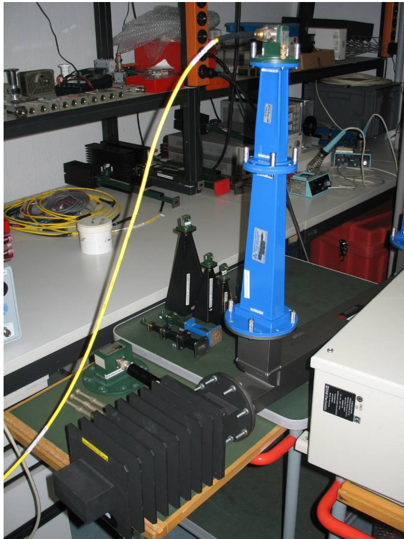
Photo No. 5: conducted measurements, spurious emissions up to 10 GHz
