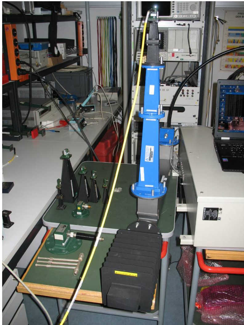
Photo No. 6: conducted measurements, spurious emissions up to 21 GHz
