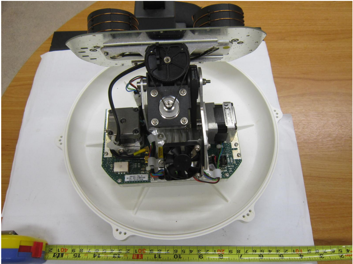
EUT Internal View
