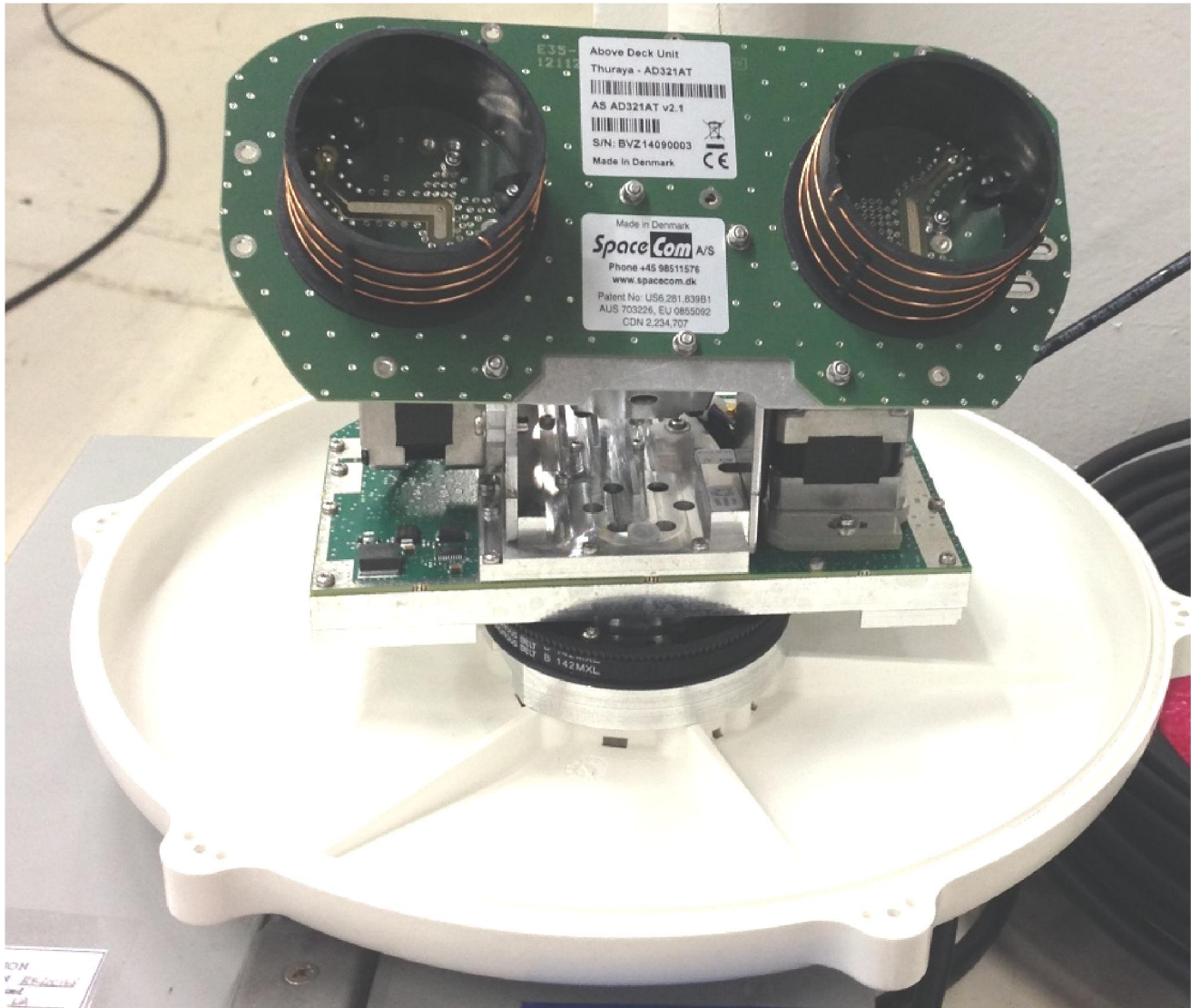
Antenna Unit Main-Board PCB Component Side
