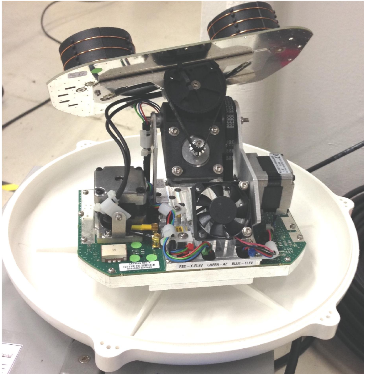
Antenna Unit Main-Board PCB Trace Side
