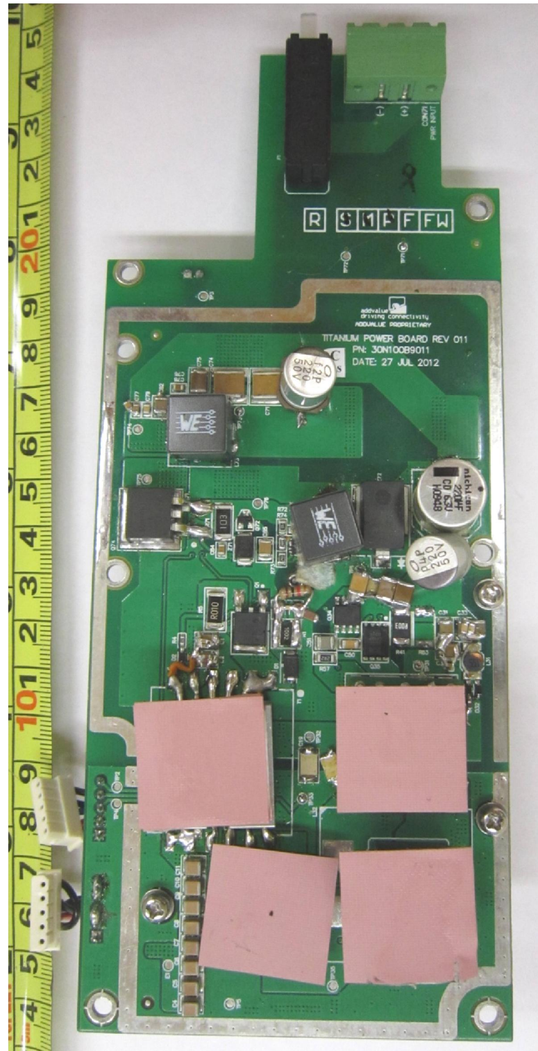
Power Supply Board PCB Component Side
