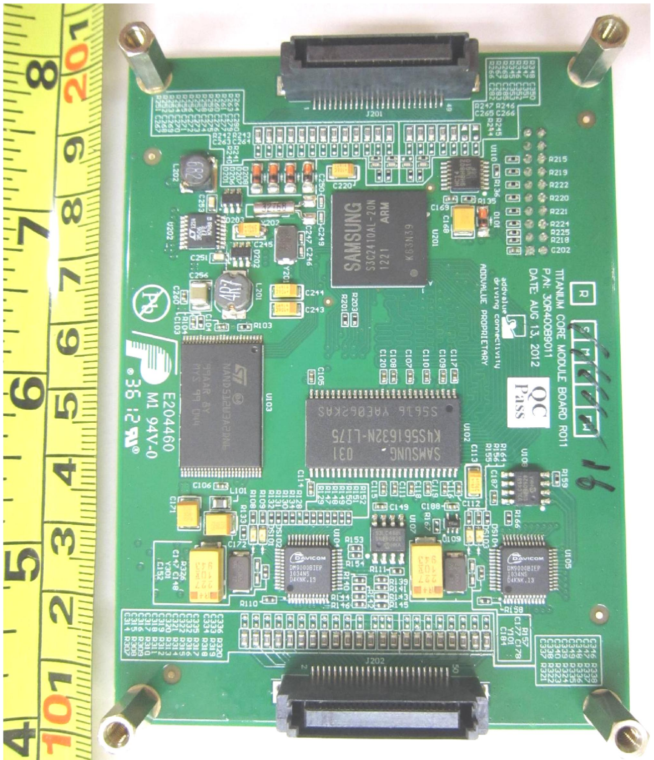
Core Module Board PCB Component Side
