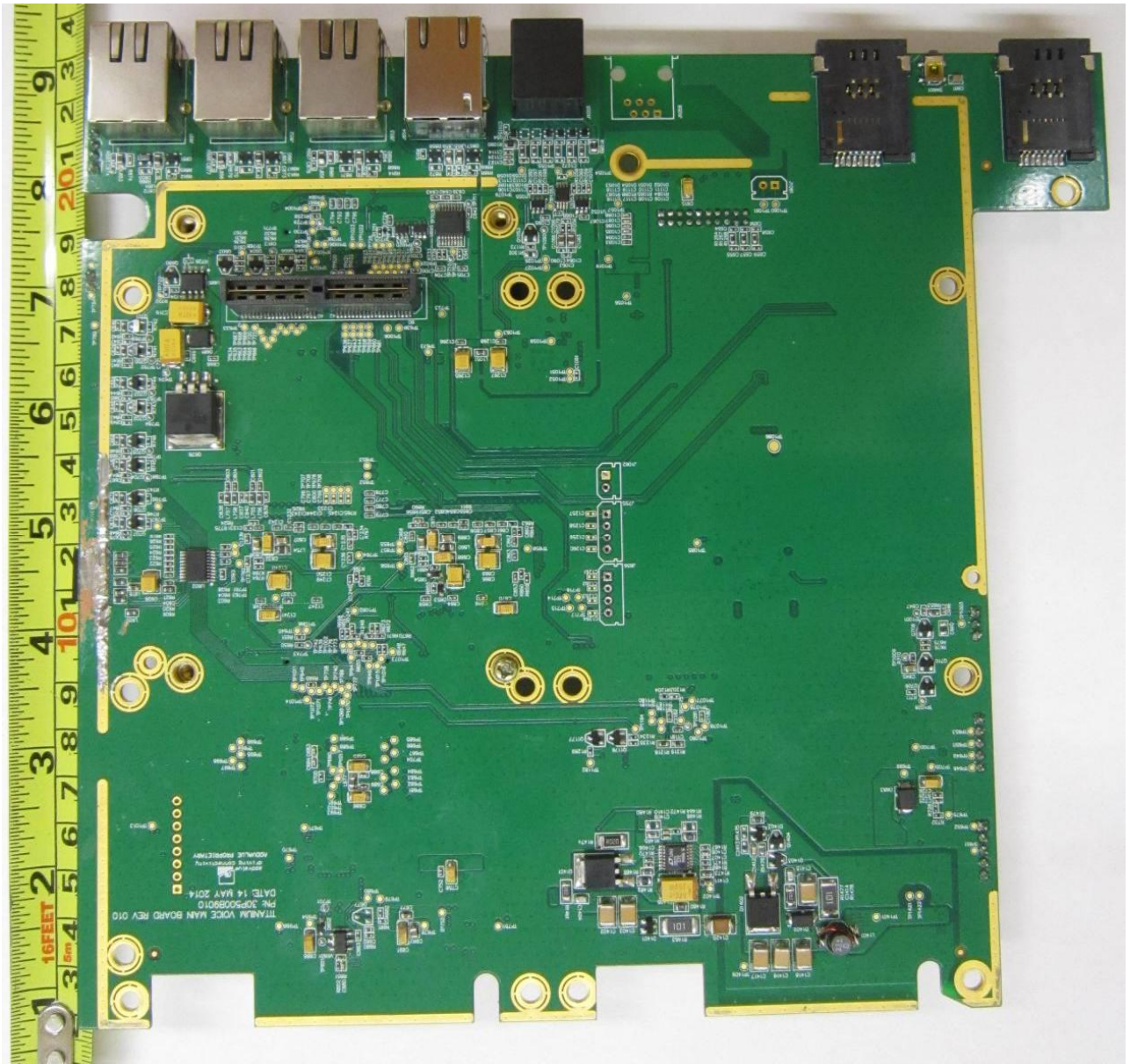
Voice Main Board PCB Component Side
