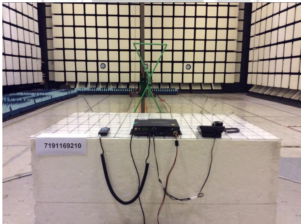
Radiated Emissions & Radiated Spurious Emissions Test Setup (Rear View)
