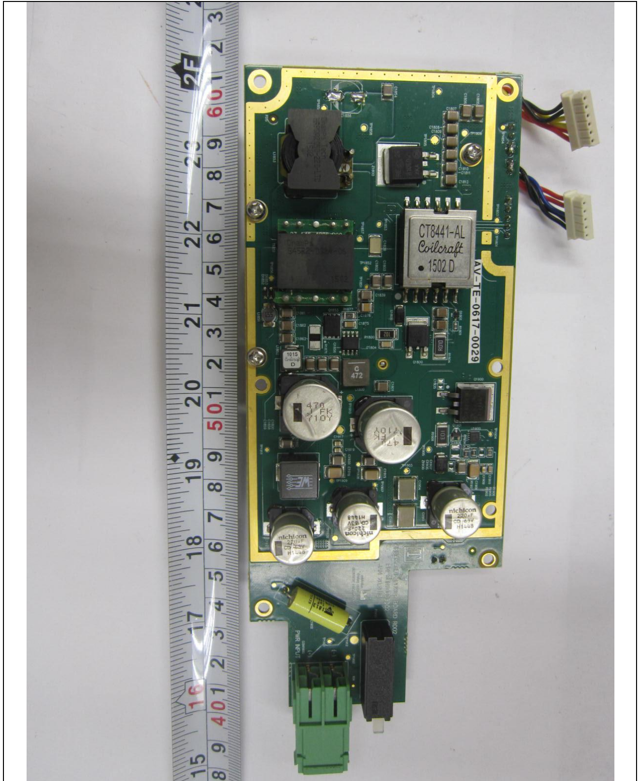
Sub-Board 2 PCB Trace View
