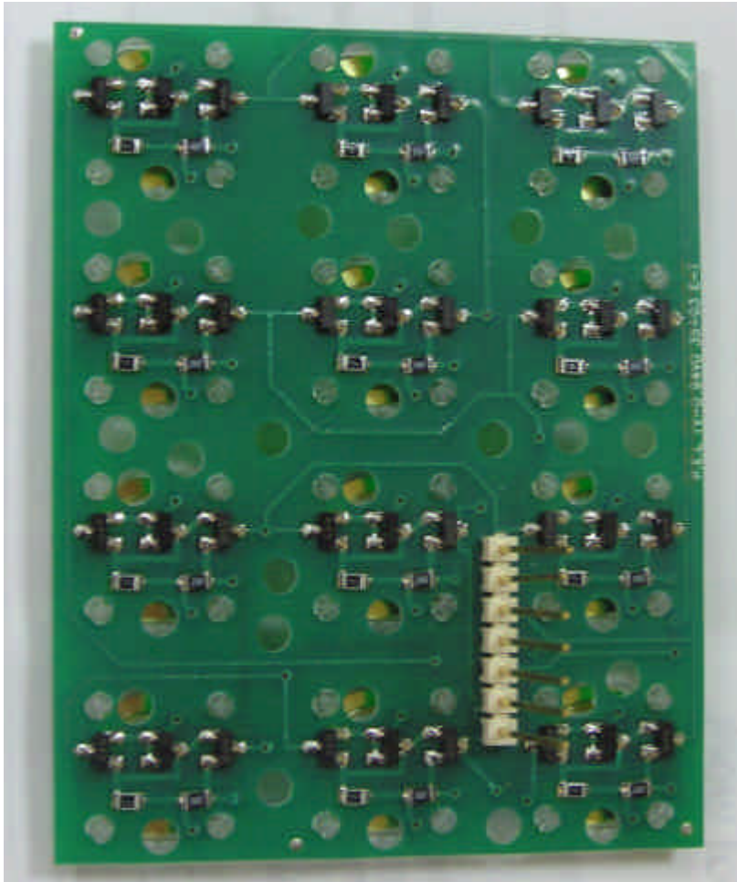
Photograph No.11 Keypad PCB front side
