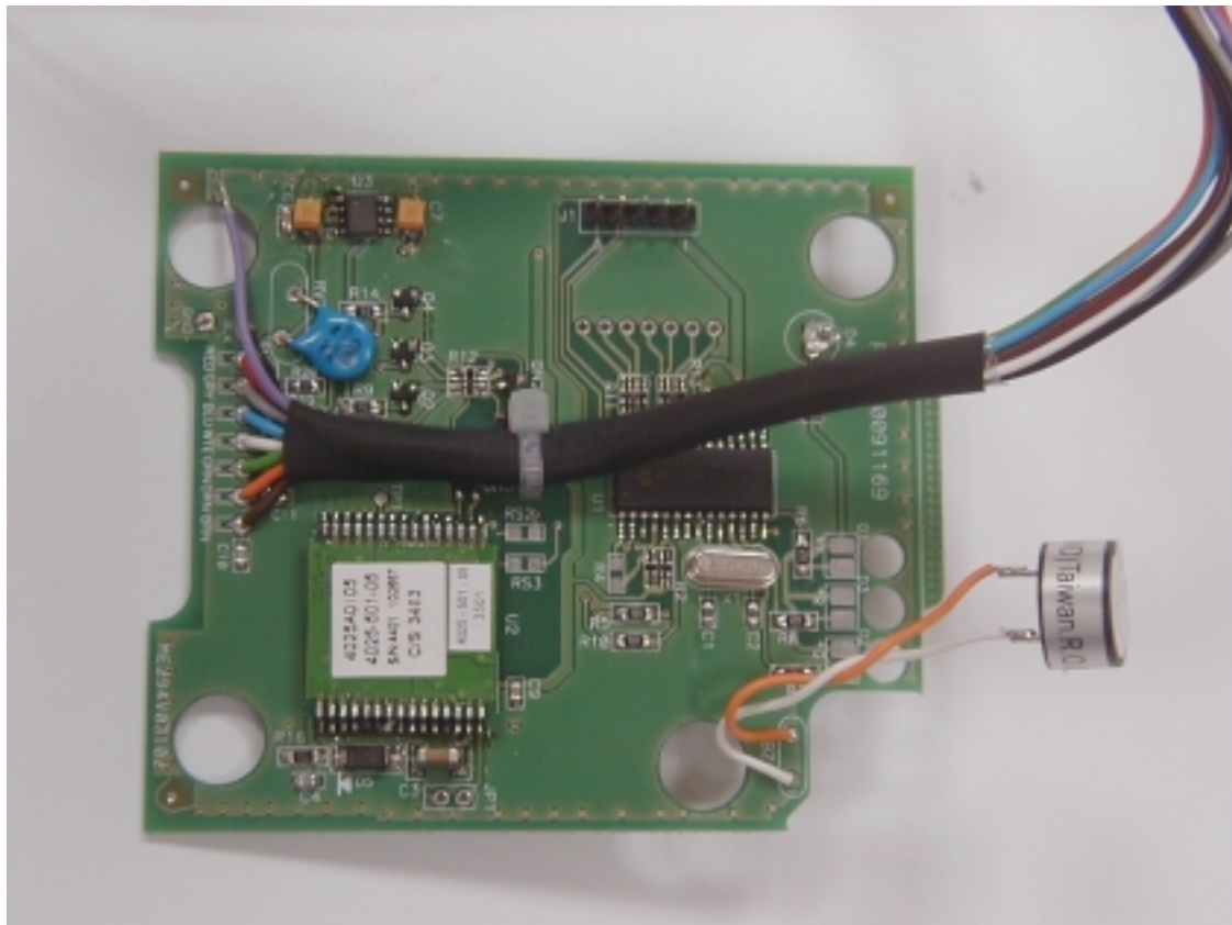
Small PCB, first side
