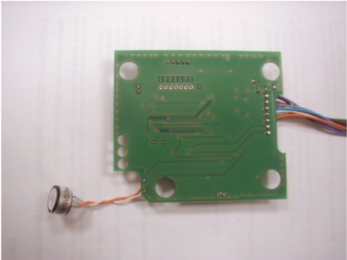
Small PCB, second side
