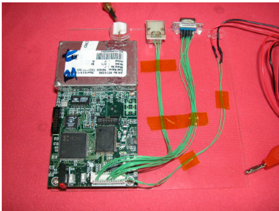
Main PCB comp side (view 1)
