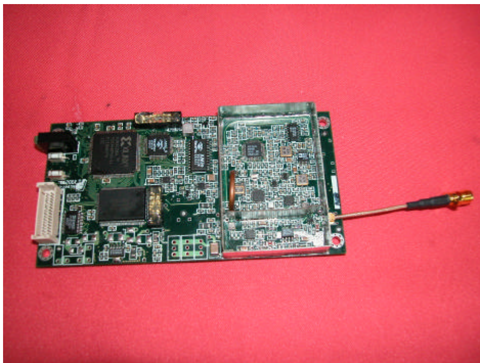
Assembly (View 1)
