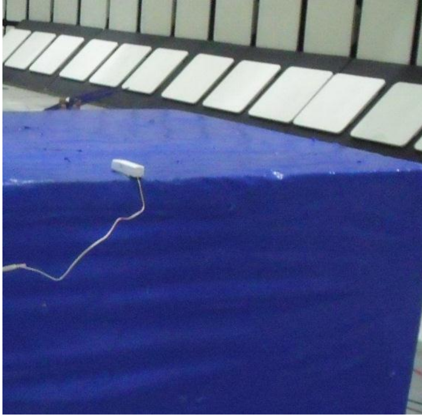
RADIATED EMISSION FOR PORTABLE CONFIGURATION – X ORIENTATION
