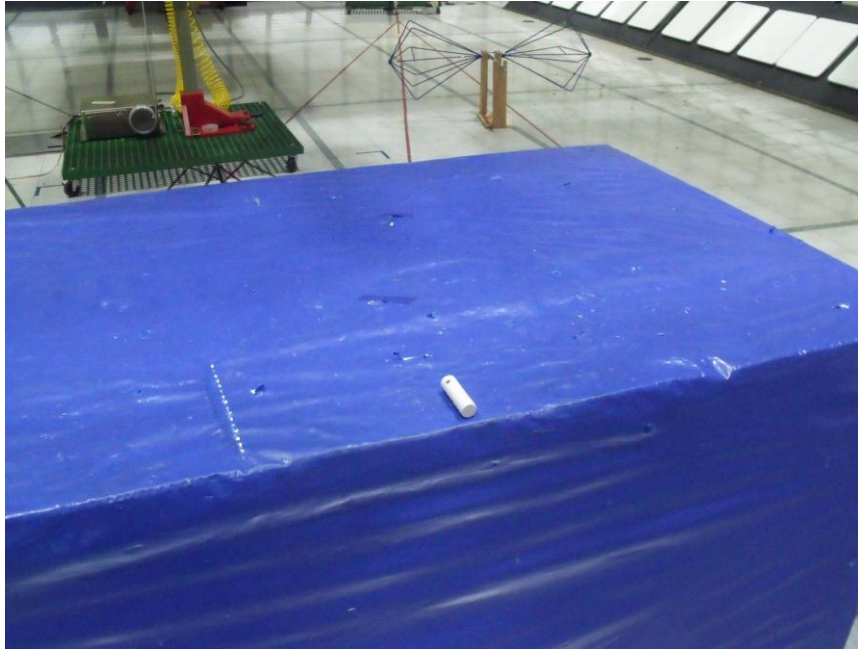
RADIATED EMISSION FOR PORTABLE CONFIGURATION – Z ORIENTATION
