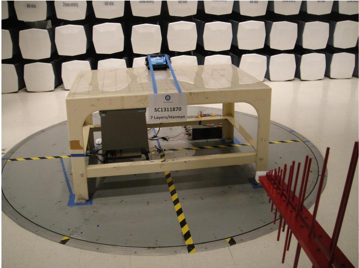
BT Radiated Emission Below 1GHz (Front)
