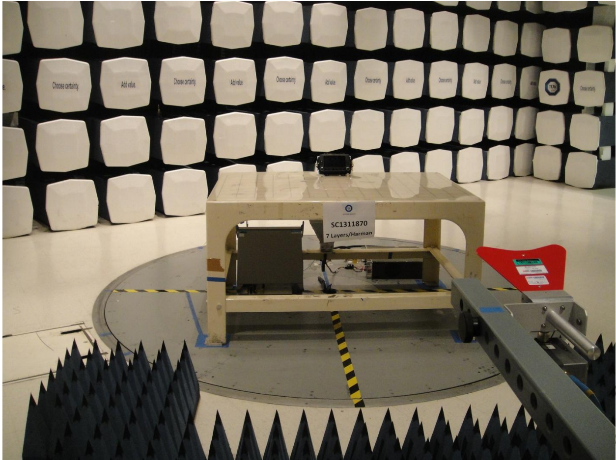
BT Radiated Emission Above 1GHz (Front)
