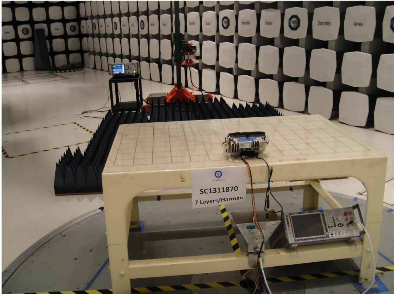
BT Radiated Emission Above 1GHz (Back)
