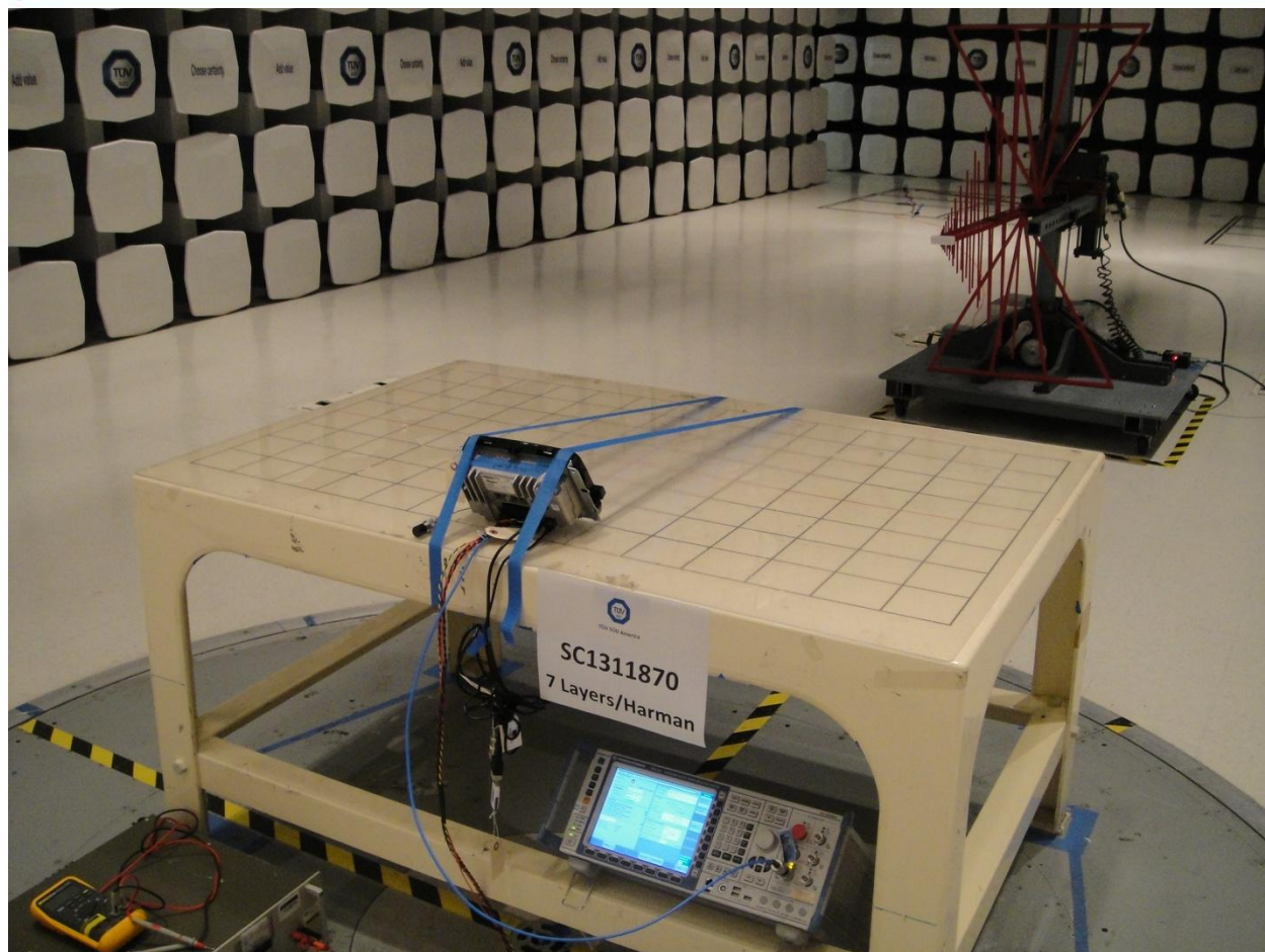
BT/WLAN Radiated Emission Below 1GHz (Back)
