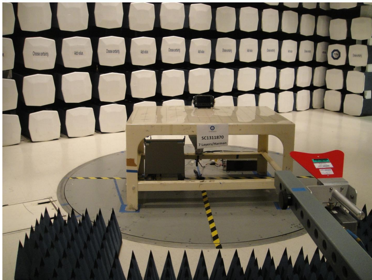
BT/WLAN Radiated Emission Above 1GHz (Front)
