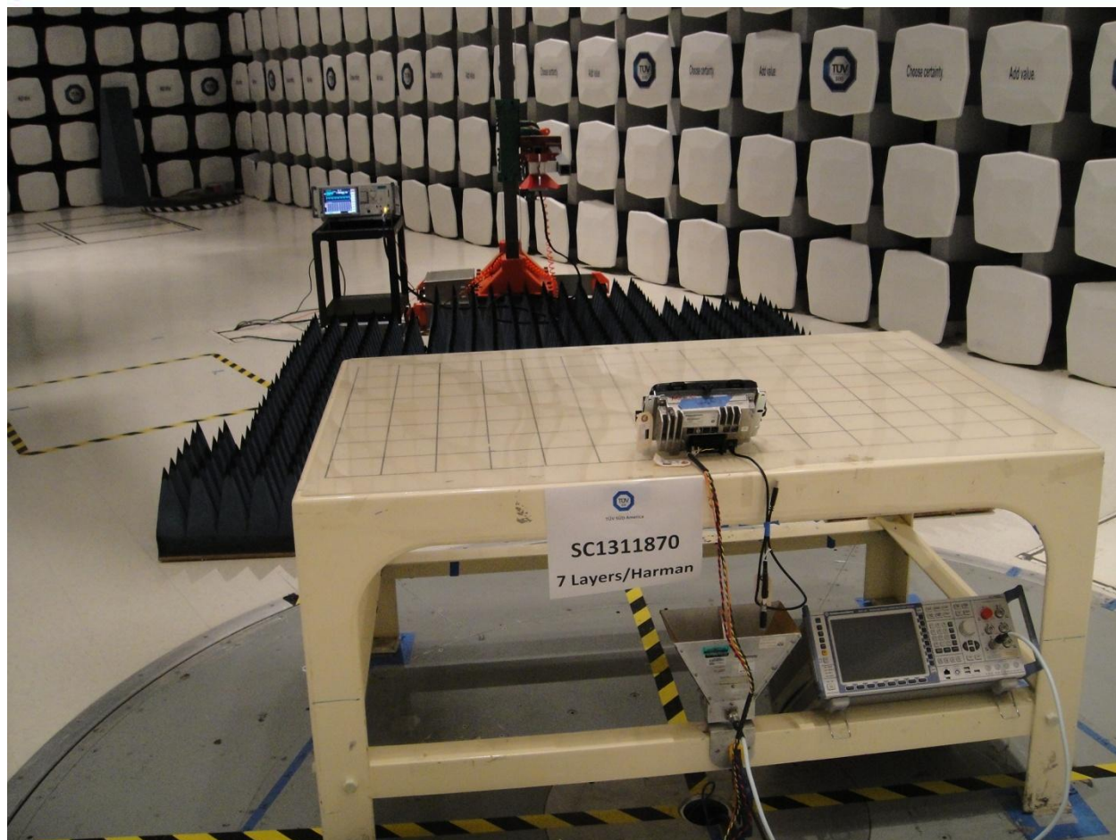
BT/WLAN Radiated Emission Above 1GHz (Back)
