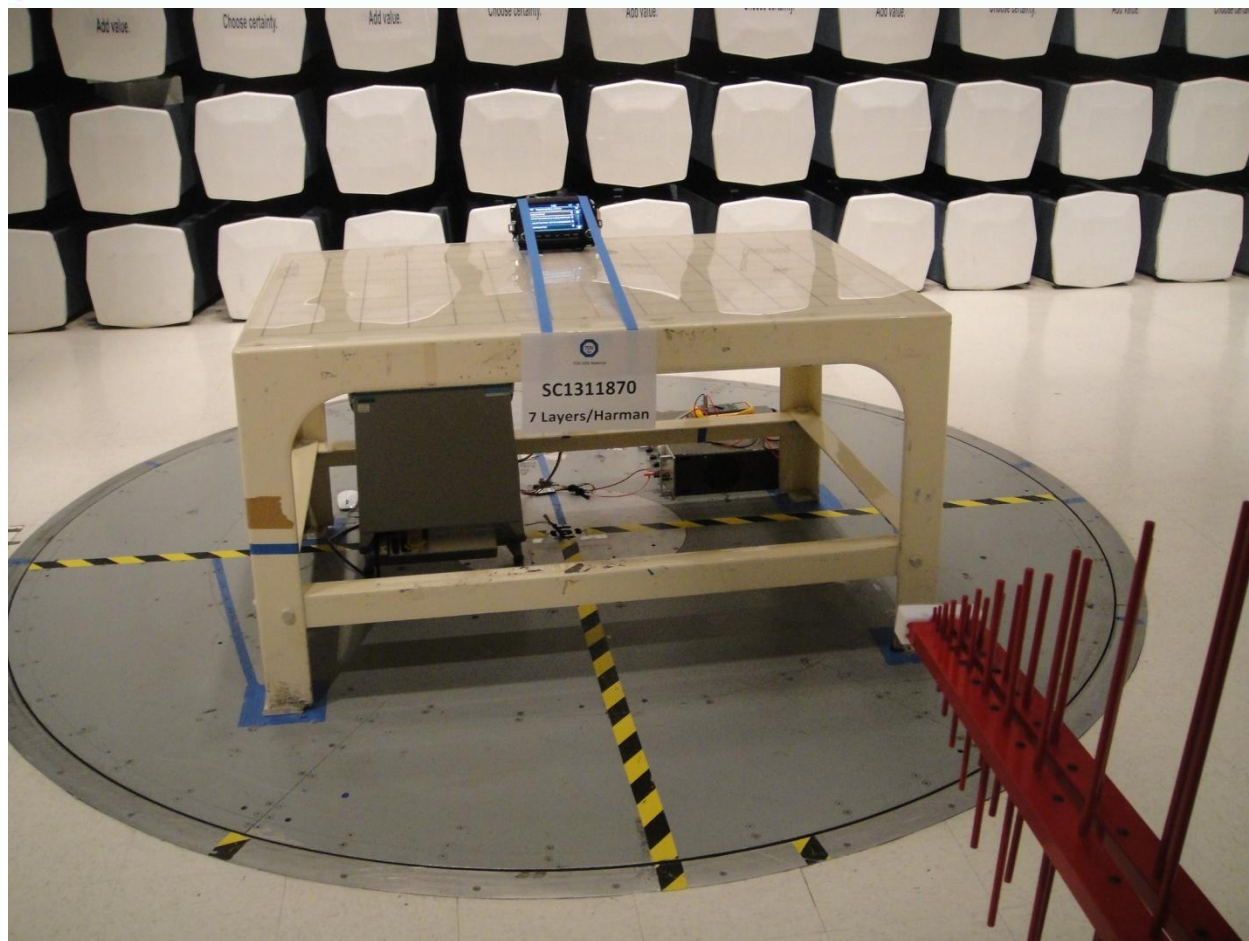
BT/WLAN Radiated Emission Below 1GHz (Front)
