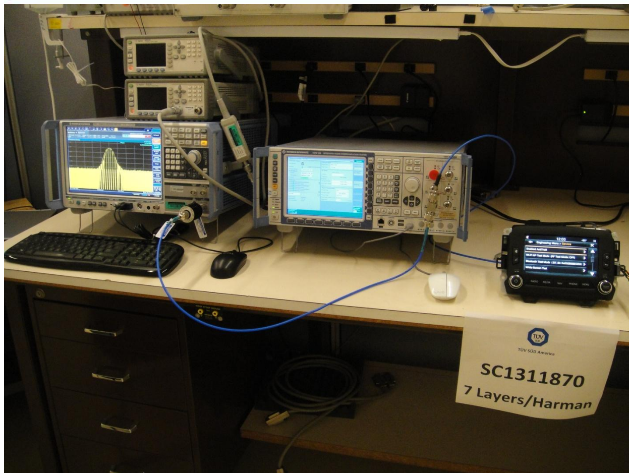
BT/WLAN Conducted Antenna Port Measurement
