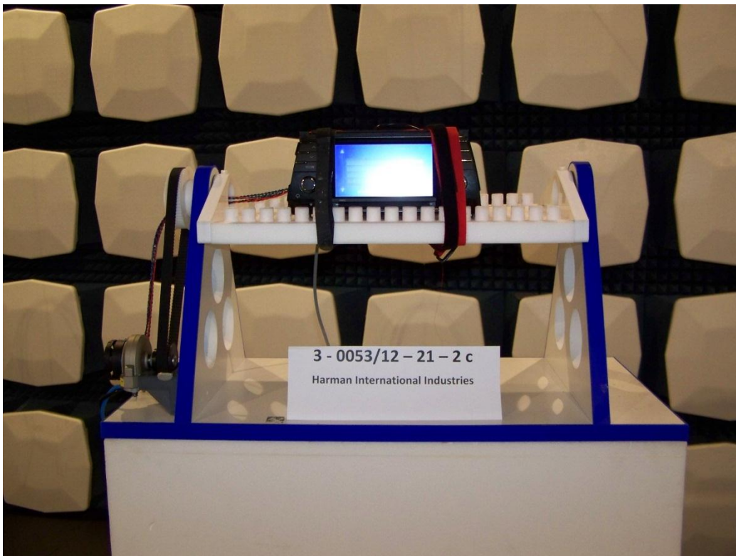
Photograph 2: Radiated measurements test set-up (Fully-Anechoic-Chamber)
