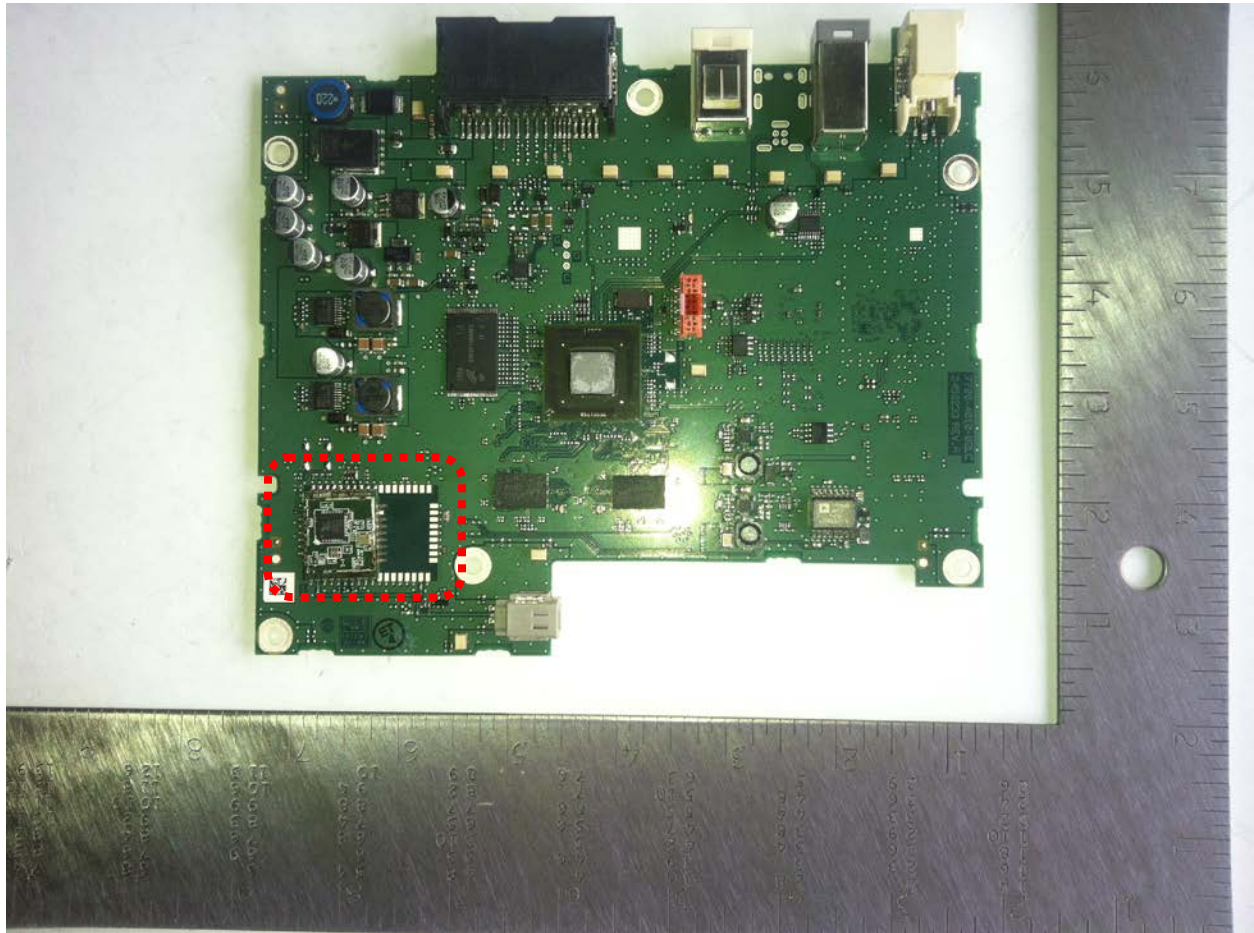
Bluetooth Transmitter (Highlighted) & All Shields Removed
