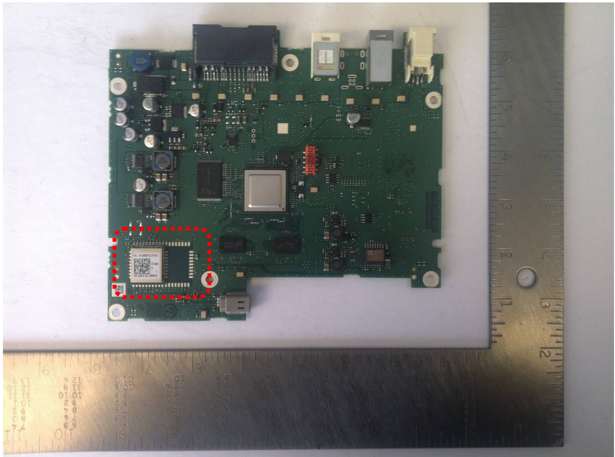
Bluetooth Transmitter (Highlighted)
