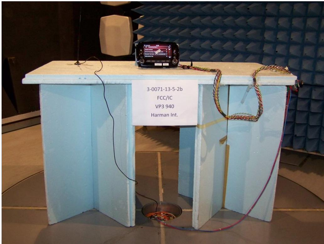
Photograph 3: Radiated measurements test set-up (Semi-Anechoic-Chamber)
