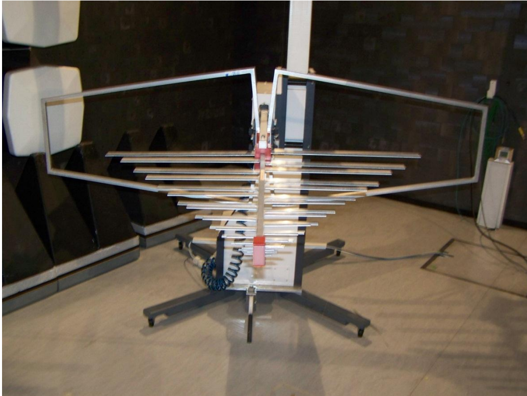
Used antenna (BTA-L ref.no 574) in the Semi Anechoic chamber (SAR)
