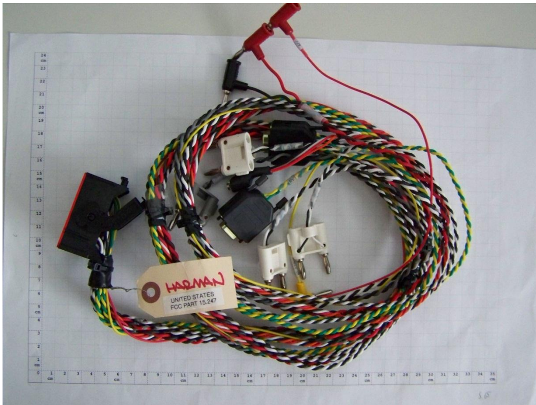
Cable 1 (Power supply cables on the upper side, double red and black plugs)
