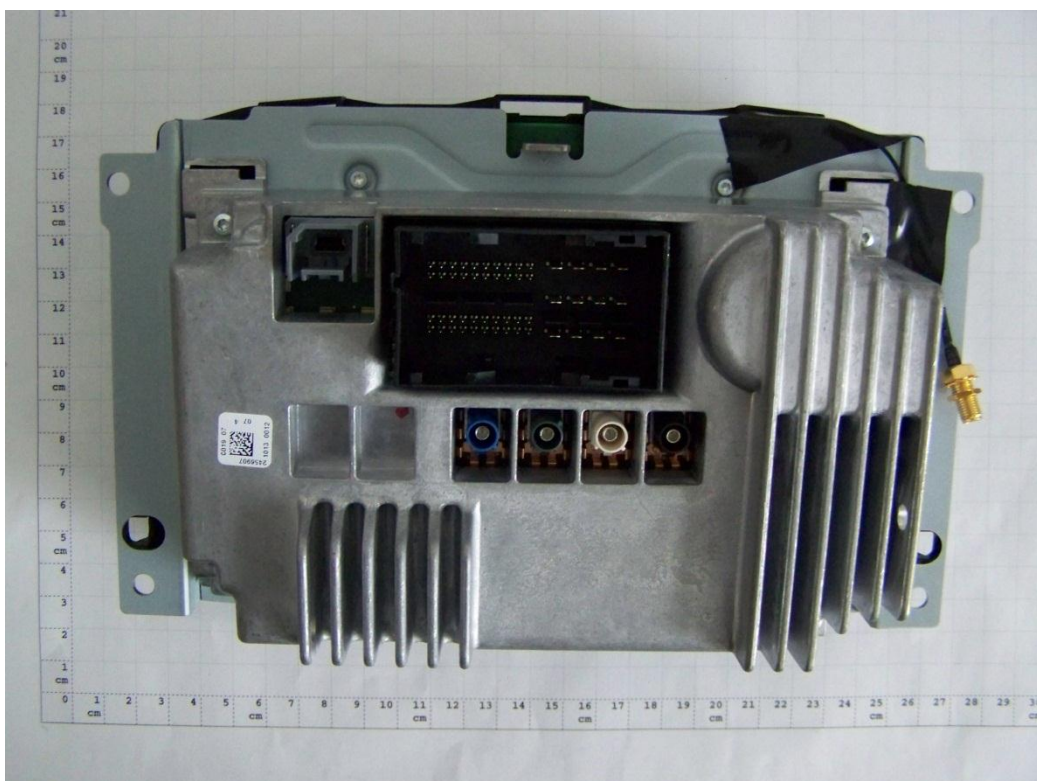
EUT C (conducted sample, Bluetooth RF cable fixed on upper right side)
