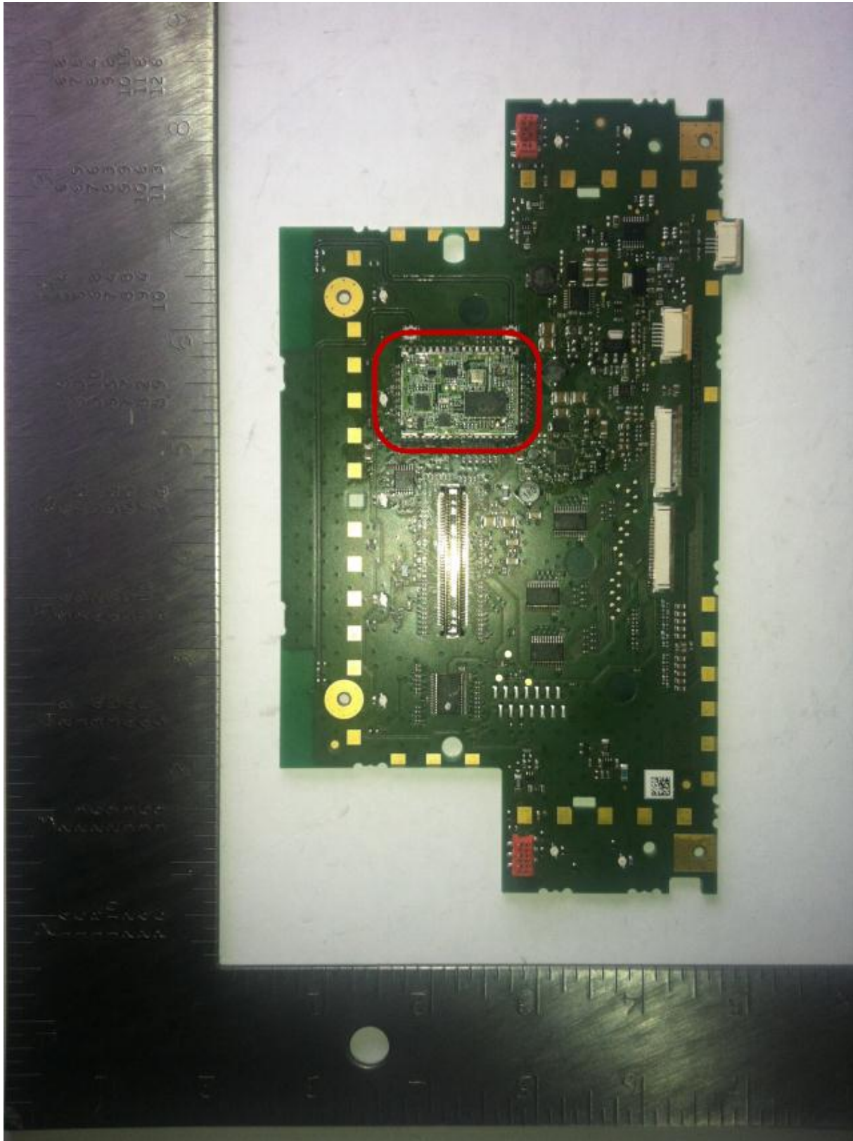
EUT inside - Bluetooth Transmitter and highlighted in red box (PCBA top view)
