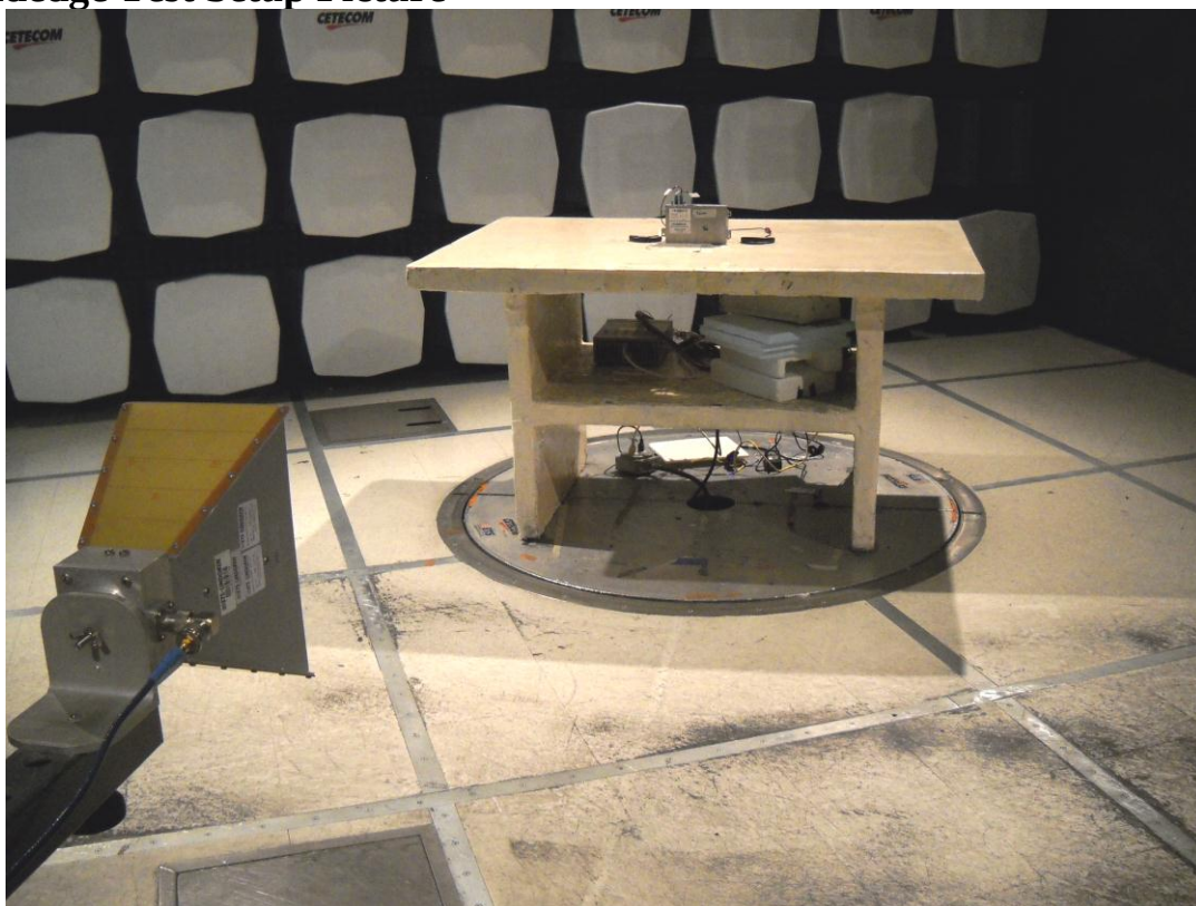
Bandedge Test Setup Picture
