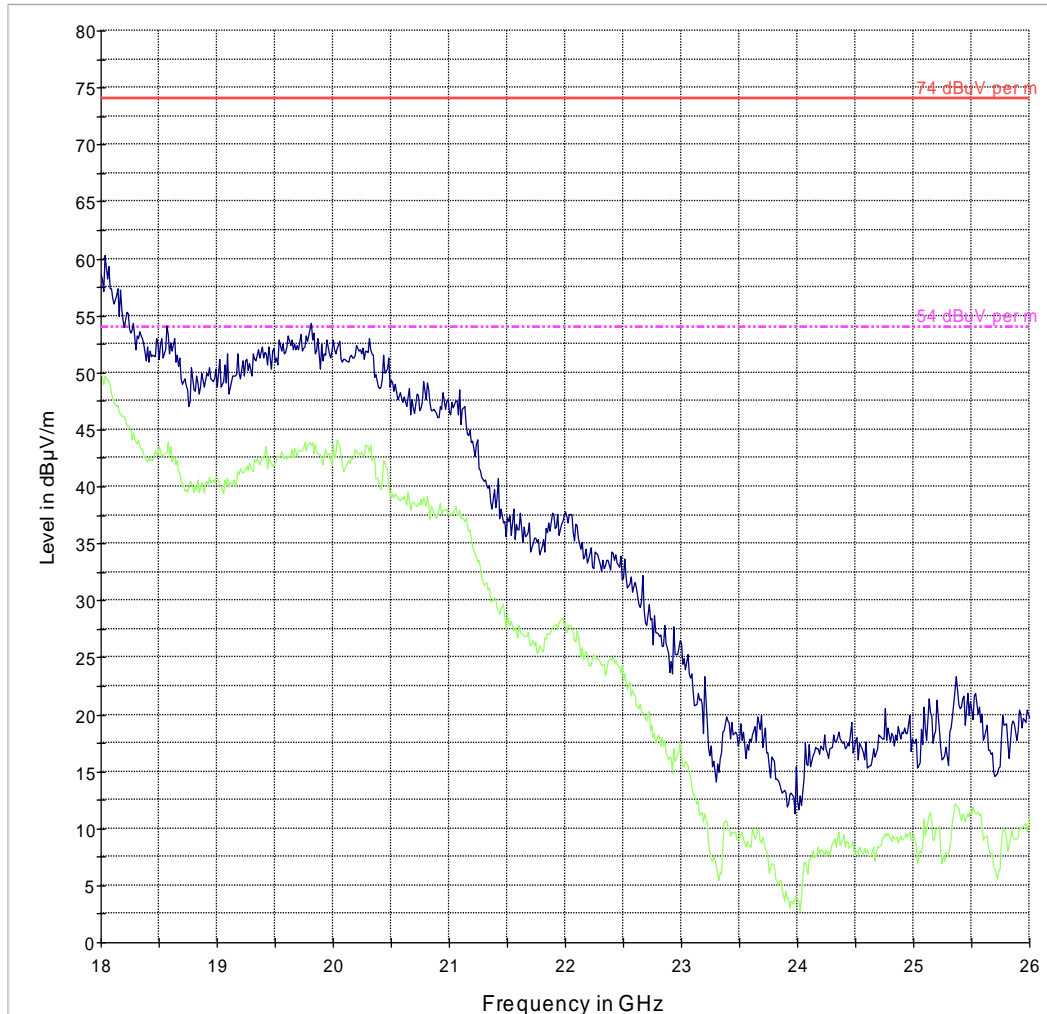
— 74 dBµV per m - - - 54 dBµV per m — Preview Result 1-PK+ — Preview Result 2-AVG
