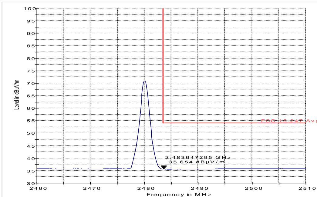
FCC 15.247 HBE Avg 3m
