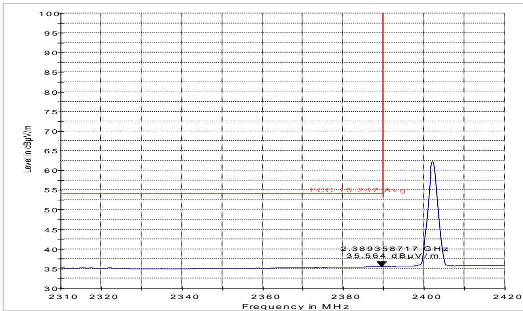
FCC 15.247 LBE Avg 3m
