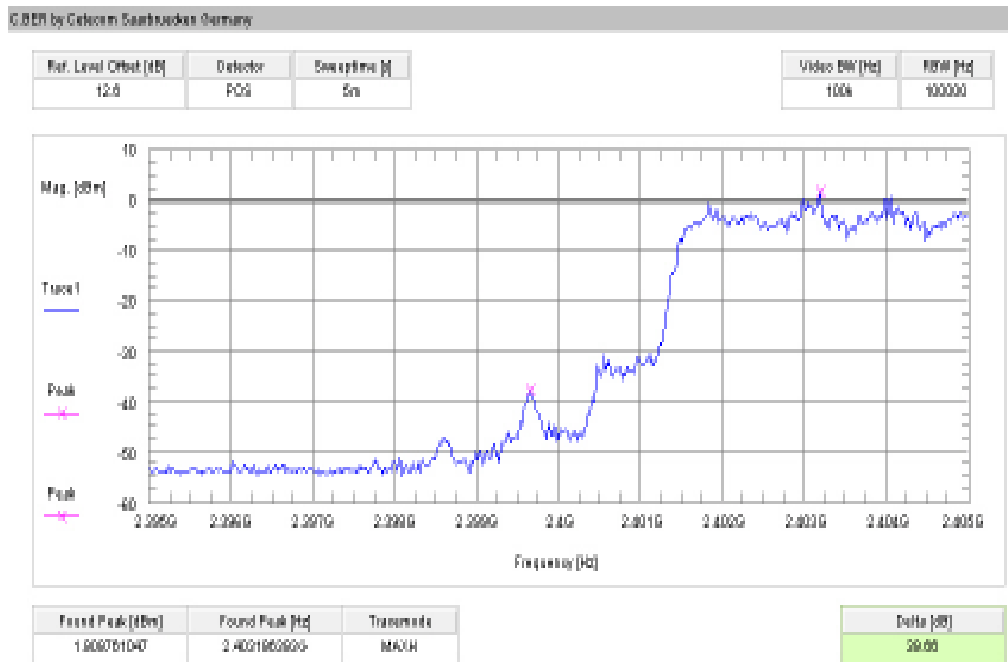
Plot 5: lower band edge – hopping on, Pi/4 DQPSK modulation (conducted)
