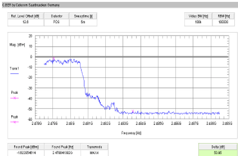
Plot 6: upper band edge – hopping on, Pi/4 DQPSK modulation (conducted)
