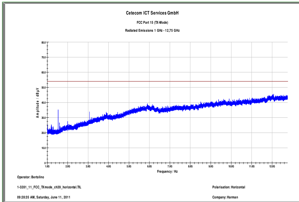
Plot 8: 1 GHz to 12.75 GHz, channel 39, horizontal polarization
