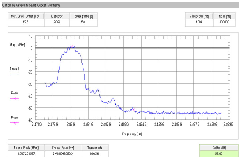
Plot 8: upper band edge – hopping off, Pi/4 DQPSK modulation (conducted)
