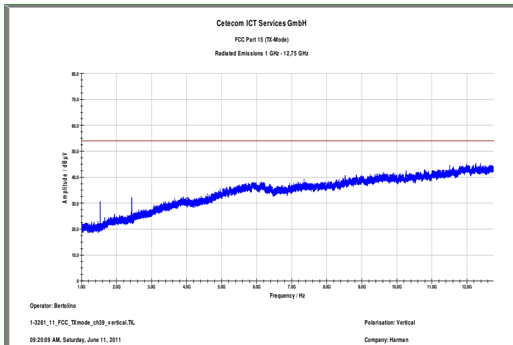
Plot 7: 1 GHz to 12.75 GHz, channel 39, vertical polarization
