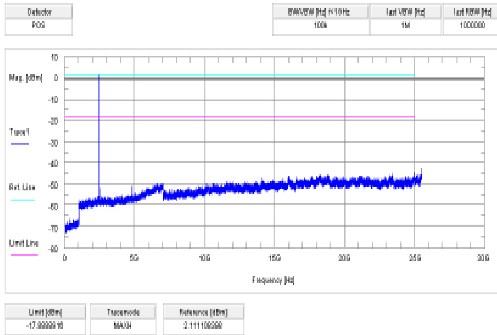
Plot 7: channel 00, 8 DPSK modulation, conducted
