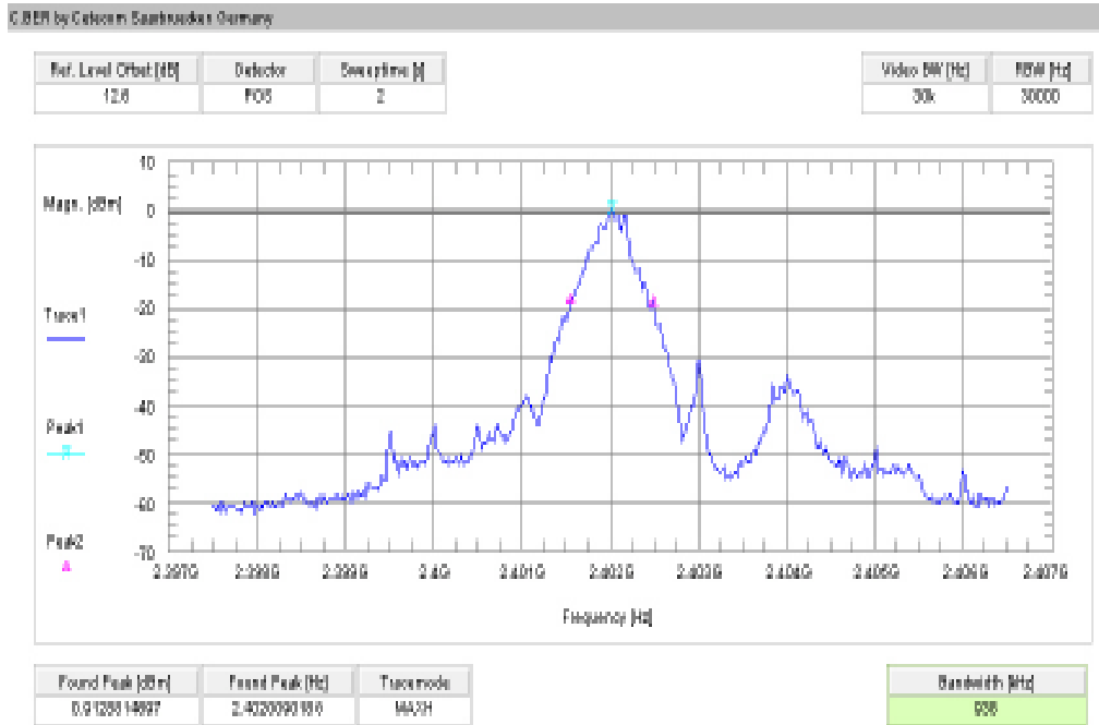
Plot 1: channel 00, GFSK modulation
