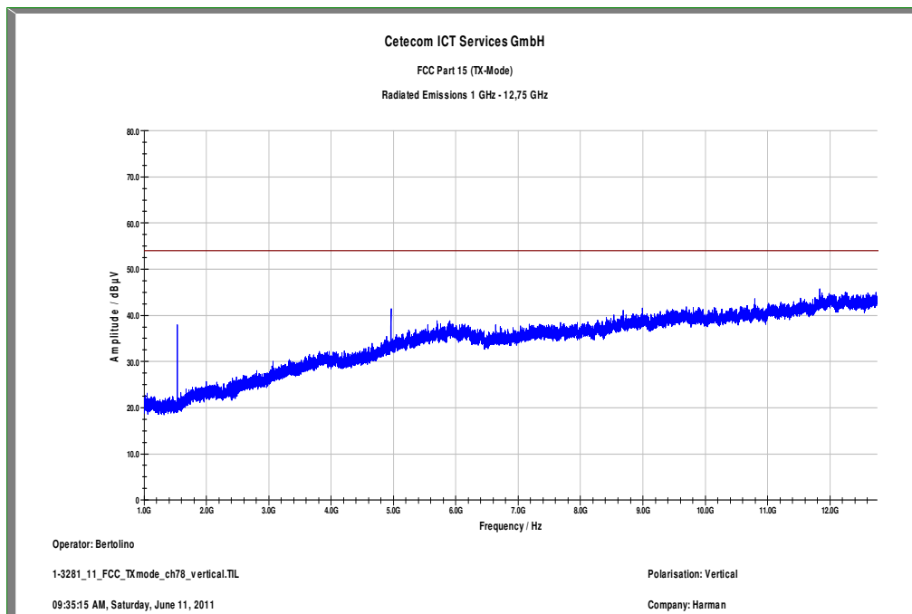
Plot 12: 1 GHz to 12.75 GHz, channel 78, vertical polarization
