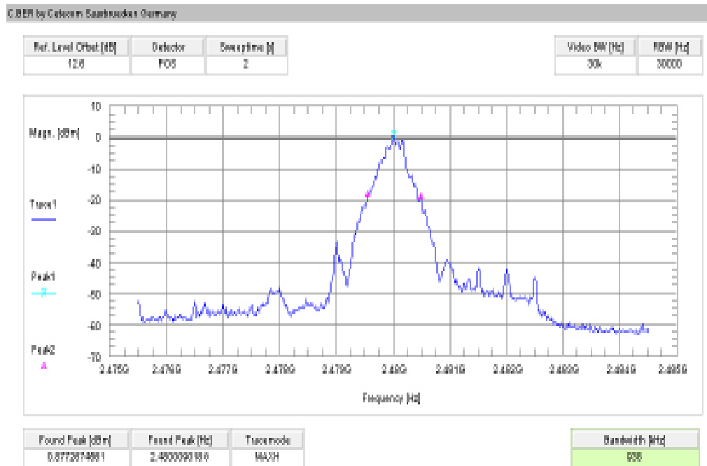
Plot 3: channel 78, GFSK modulation
