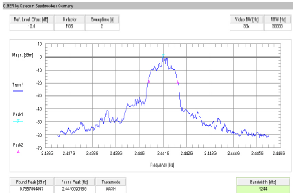
Plot 5: channel 39, Pi/4 DQPSK modulation
