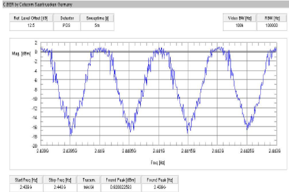
Plot 1: Carrier Frequency Separation (GFSK)
