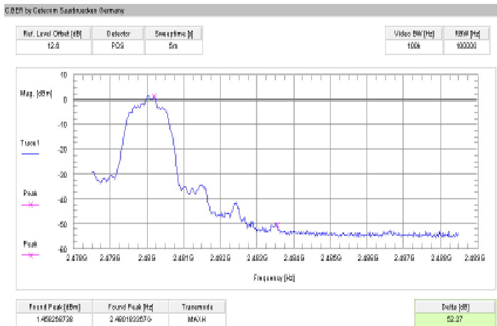
Plot 12: upper band edge – hopping off, 8 DPSK modulation (conducted)
