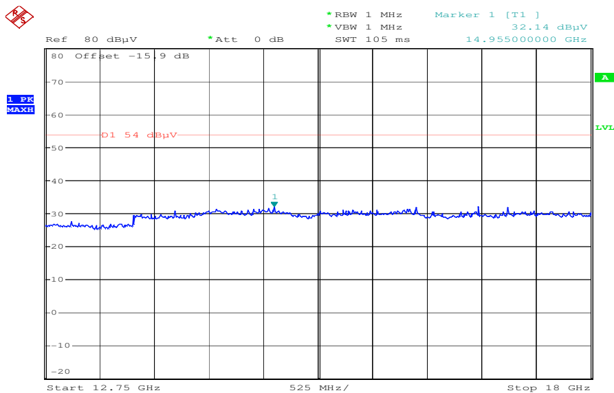
Plot 9: 12.75 GHz to 18 GHz, channel 39, vertical & horizontal polarization
