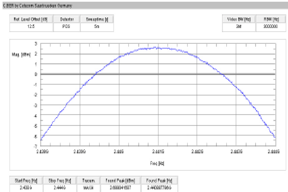
Plot 5: channel 39, Pi/4 DQPSK modulation, conducted
