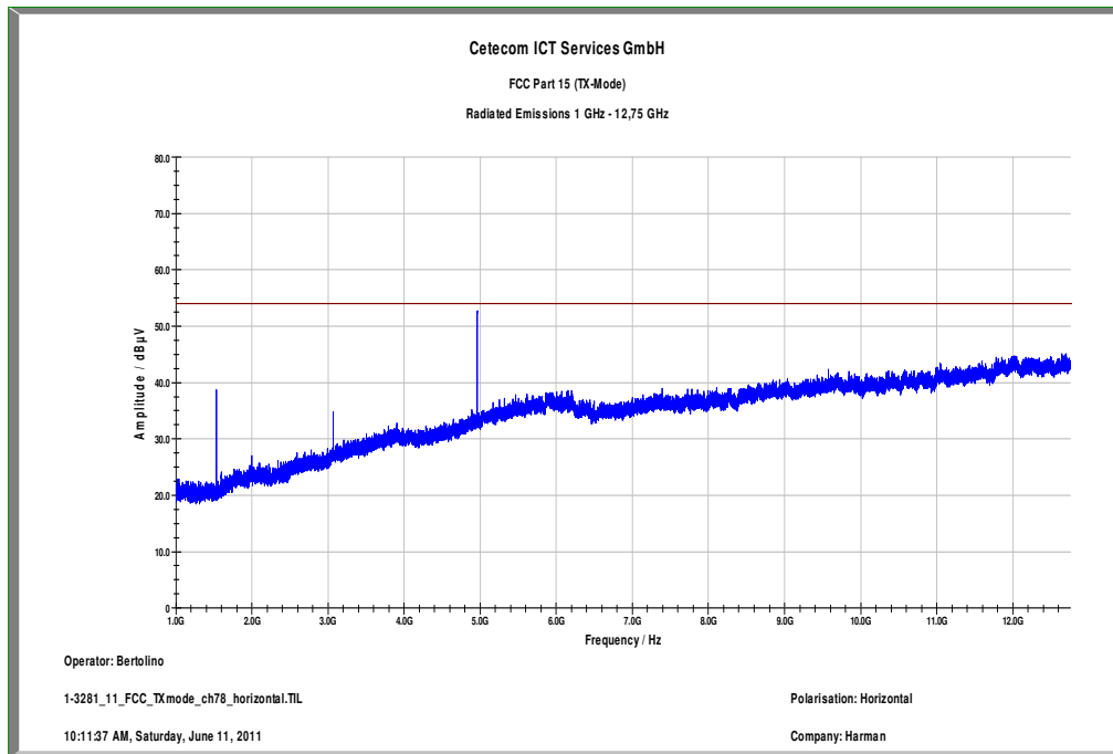
Plot 13: 1 GHz to 12.75 GHz, channel 78, horizontal polarization
