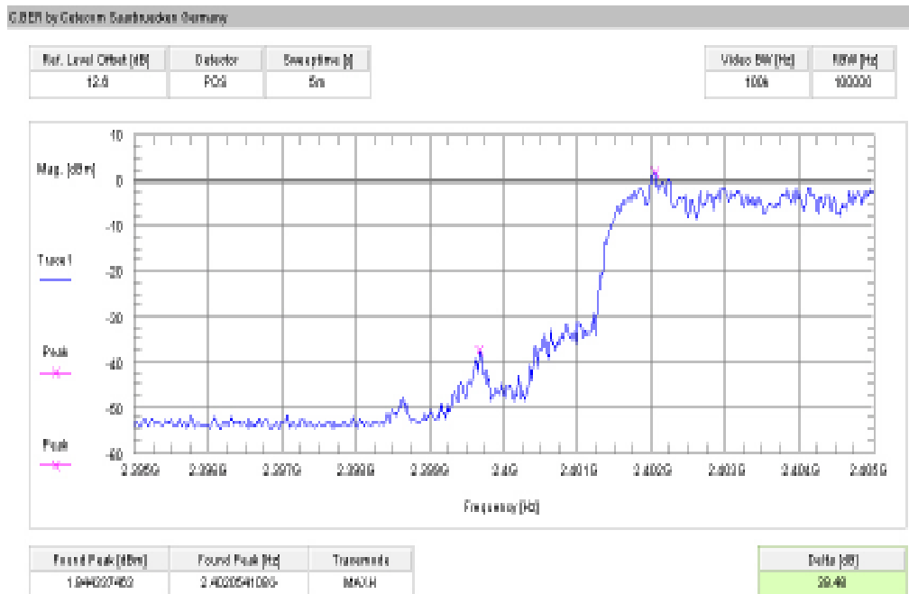
Plot 9: lower band edge – hopping on, 8 DPSK modulation (conducted)
