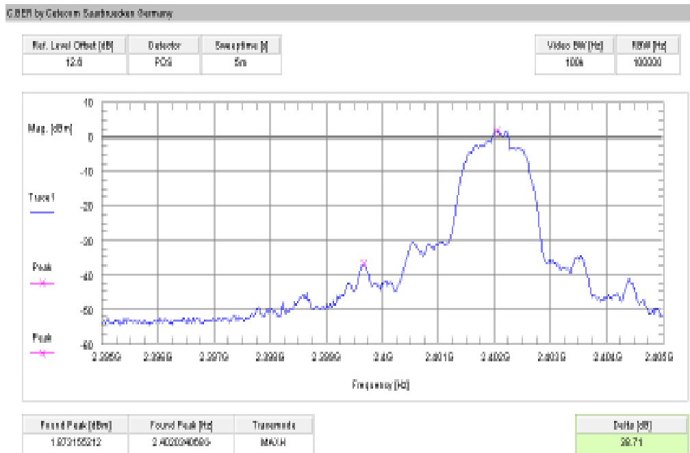
Plot 11: lower band edge – hopping off, 8 DPSK modulation (conducted)
