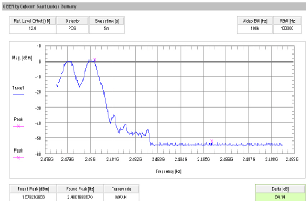
Plot 2: upper band edge – hopping on, GFSK modulation (conducted)
