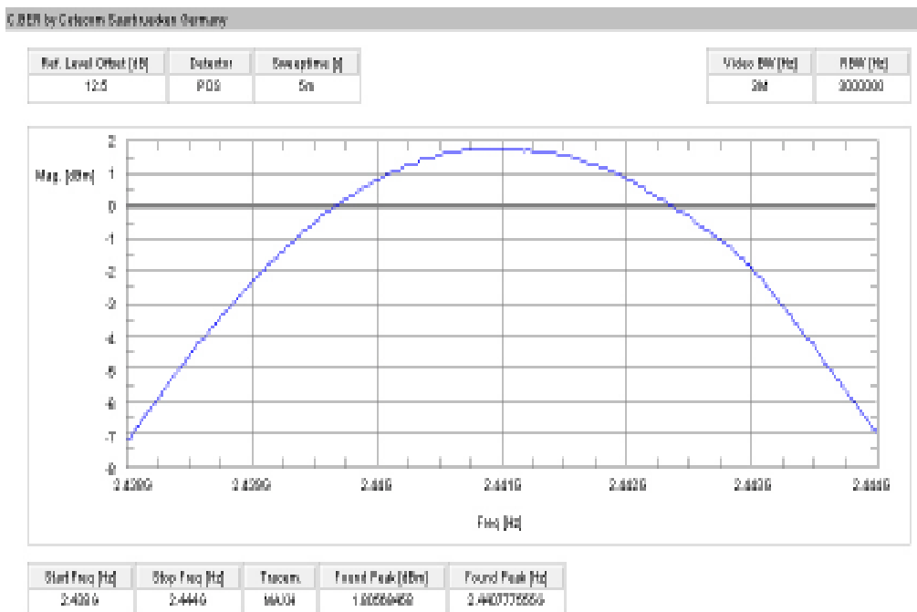
Plot 2: channel 39, GFSK modulation, conducted
