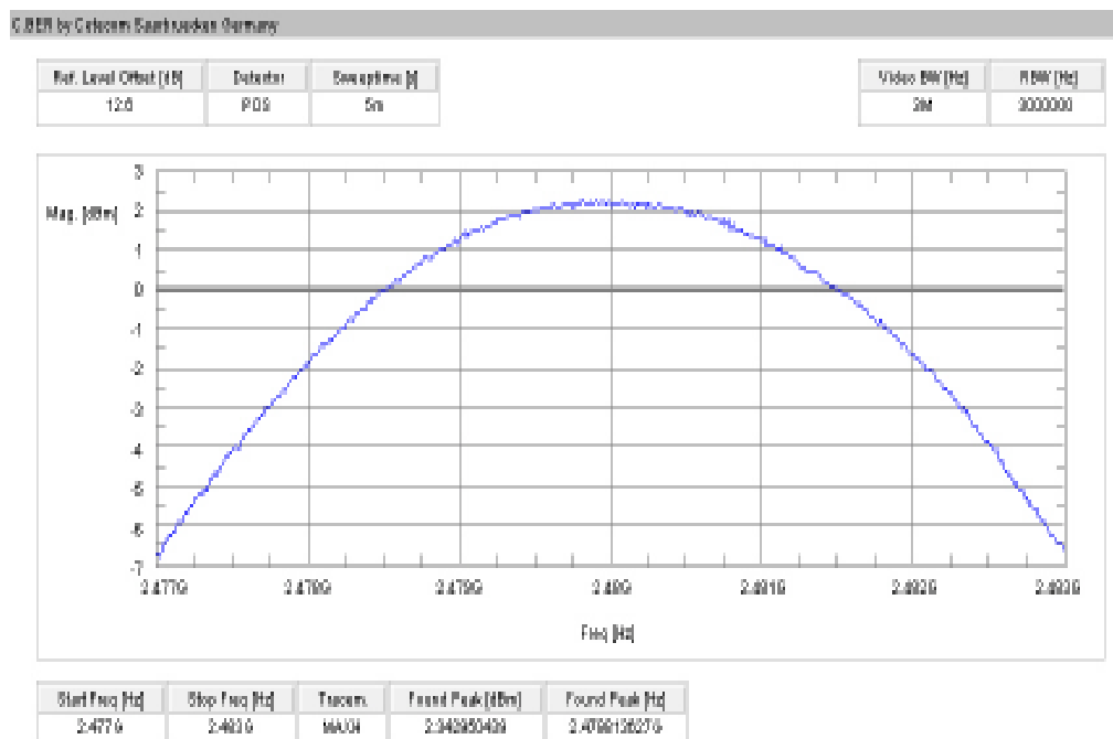
Plot 6: channel 78, Pi/4 DQPSK modulation, conducted
