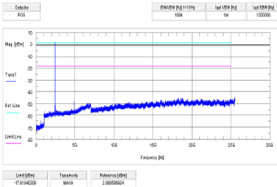
Plot 8: channel 39, 8 DPSK modulation, conducted
