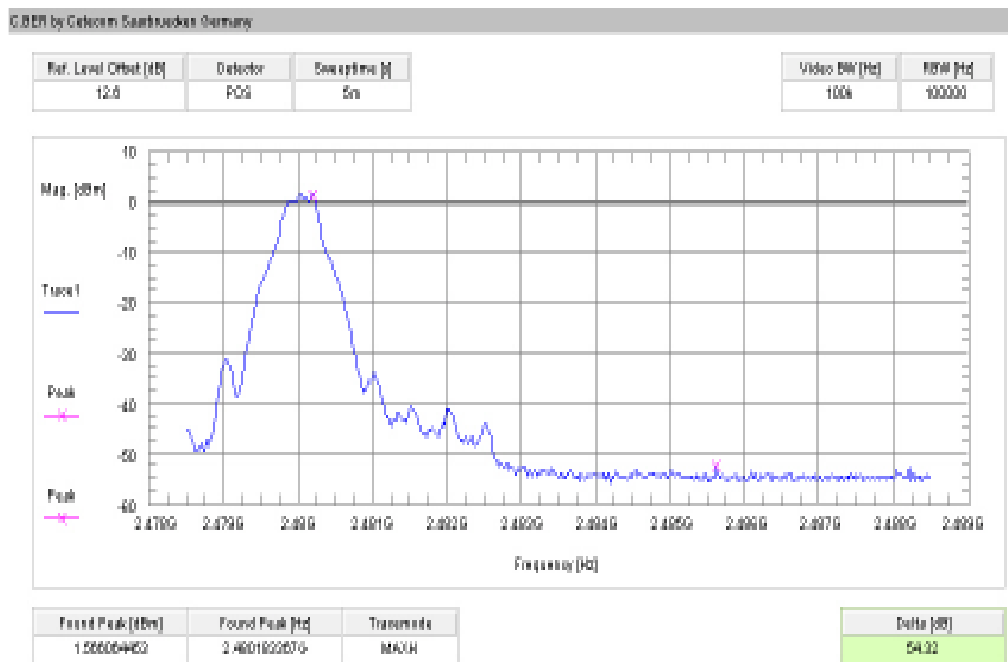
Plot 4: upper band edge – hopping off, GFSK modulation (conducted)
