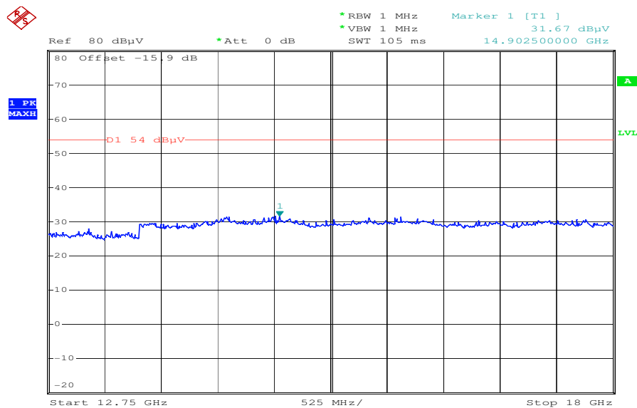
Plot 14: 12.75 GHz to 18 GHz, channel 78, vertical & horizontal polarization
