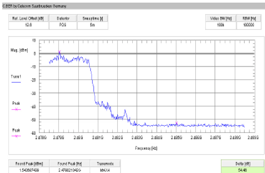
Plot 10: upper band edge – hopping on, 8 DPSK modulation (conducted)
