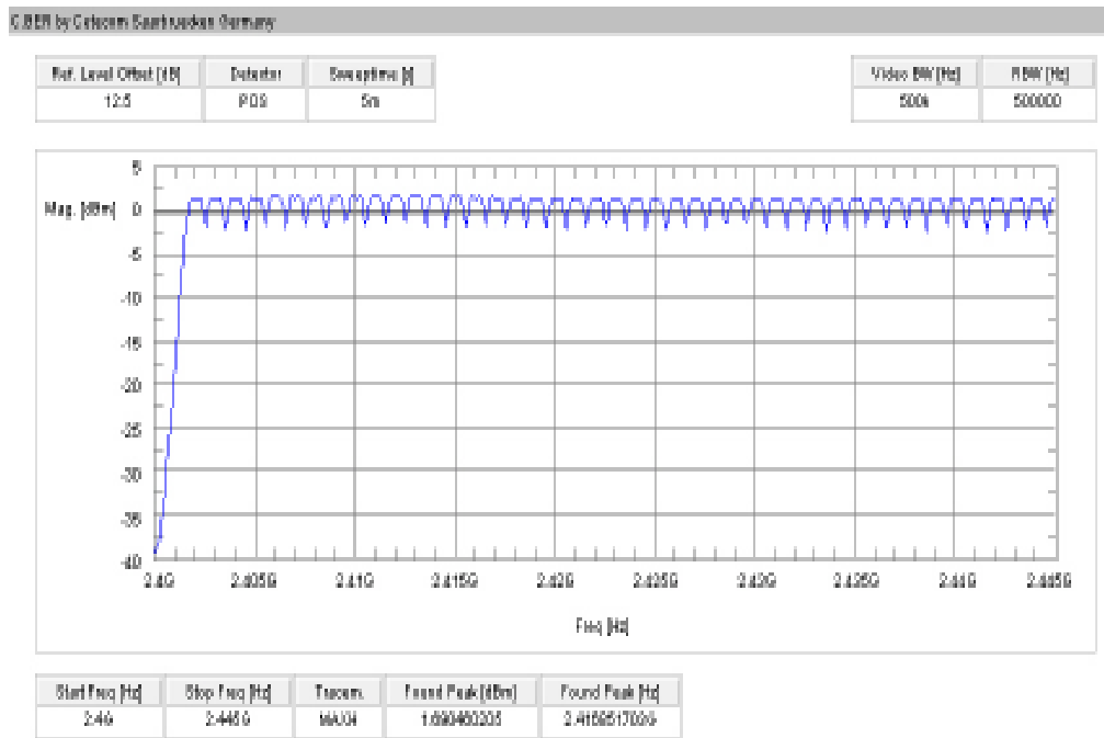
Plot 1: Number of hopping channels (GFSK)
