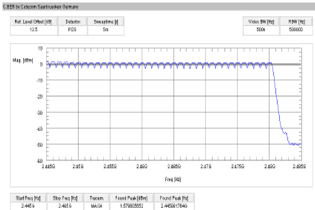
Plot 2: Number of hopping channels (GFSK)
