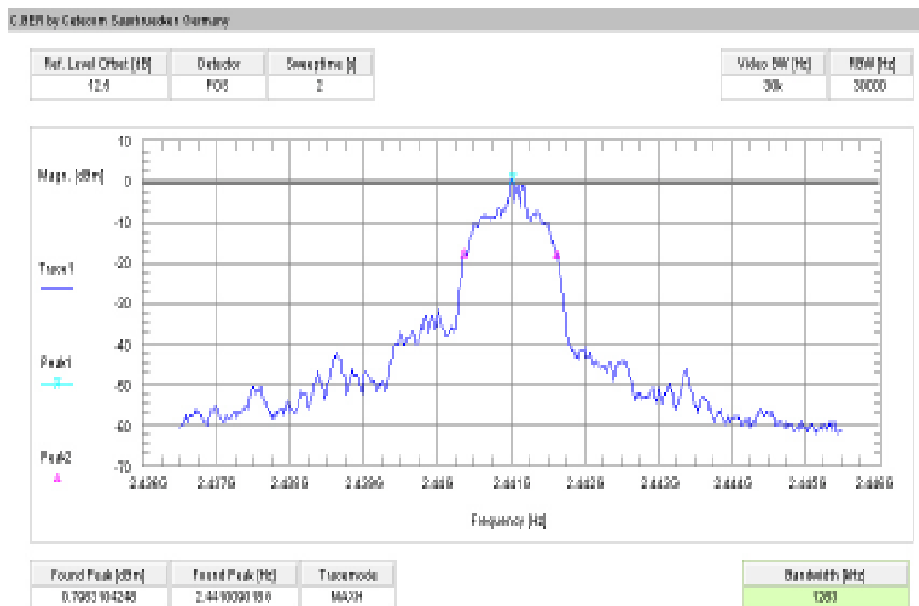
Plot 8: channel 39, 8 DPSK modulation
