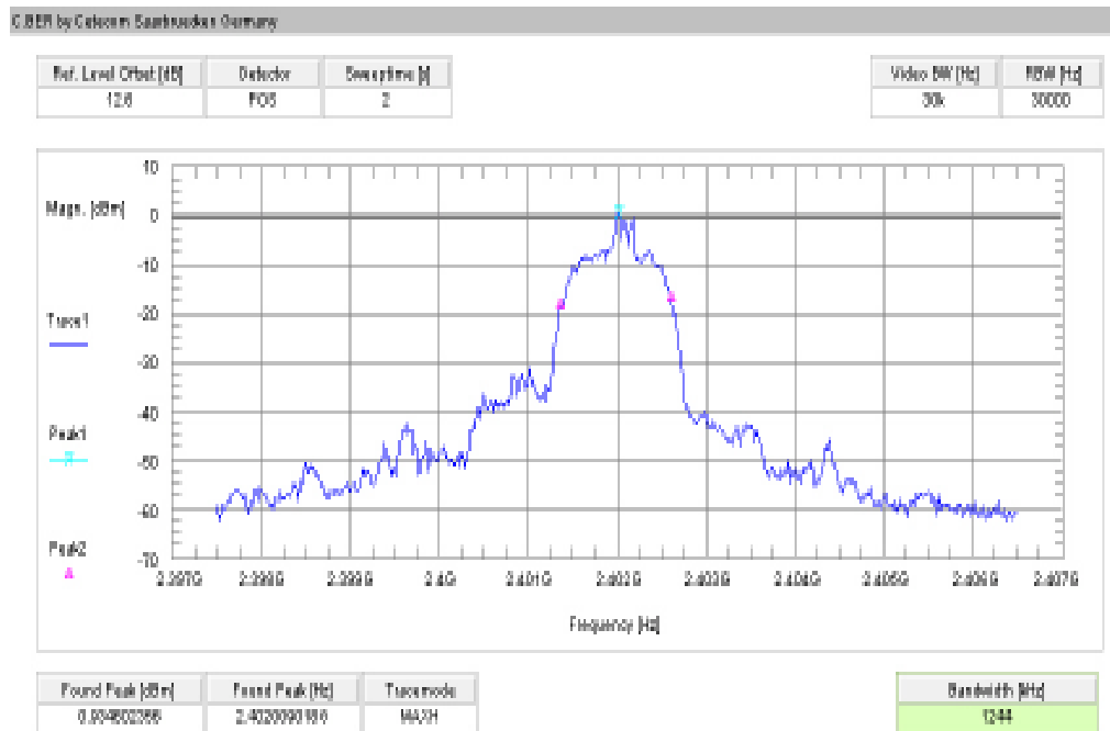
Plot 7: channel 00, 8 DPSK modulation
