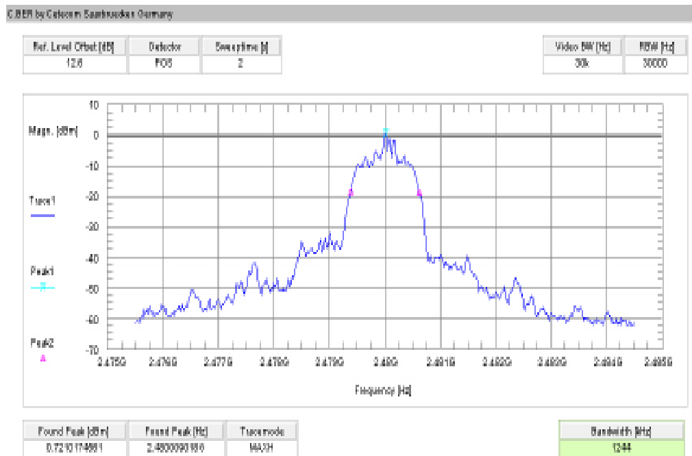
Plot 6: channel 78, Pi/4 DQPSK modulation
