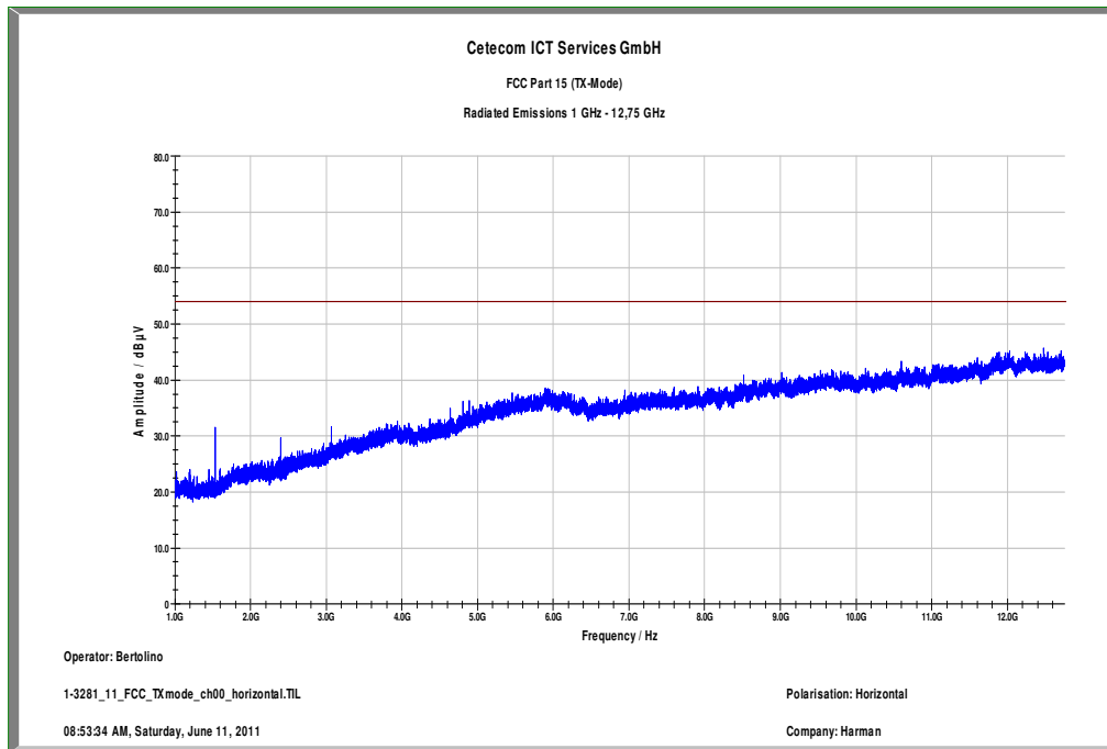
Plot 3: 1 GHz to 12.75 GHz, channel 00, horizontal polarization
