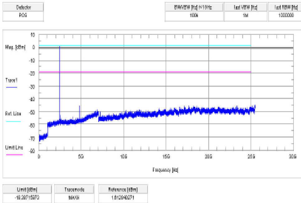
Plot 1: channel 00, GFSK modulation, conducted
