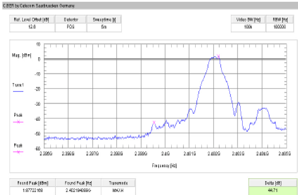
Plot 3: lower band edge – hopping off, GFSK modulation (conducted)
