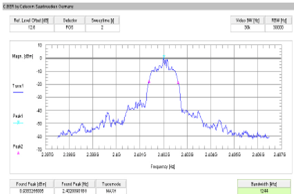
Plot 4: channel 00, Pi/4 DQPSK modulation
