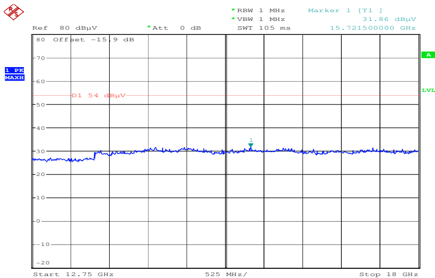
Plot 4: 12.75 GHz to 18 GHz, channel 00, vertical & horizontal polarization
