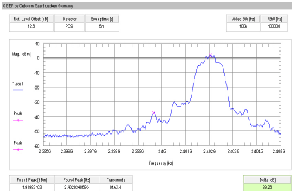
Plot 7: lower band edge – hopping off, Pi/4 DQPSK modulation (conducted)
