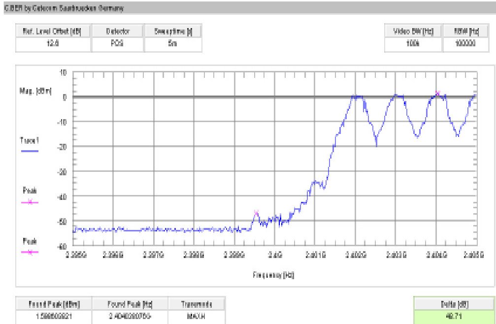
Plot 1: lower band edge – hopping on, GFSK modulation (conducted)
