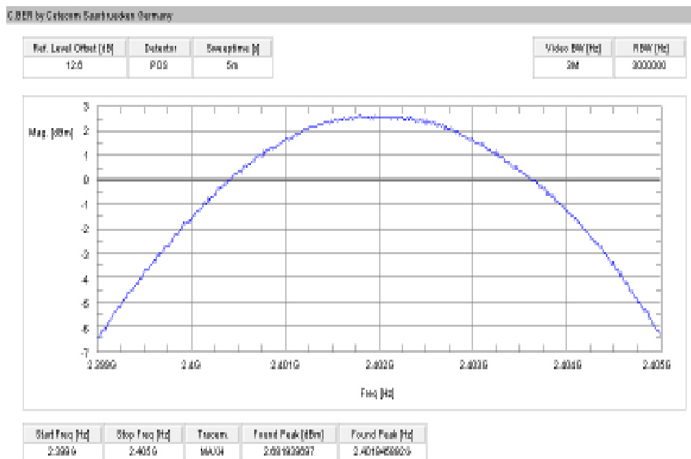
Plot 4: channel 00, Pi/4 DQPSK modulation, conducted
