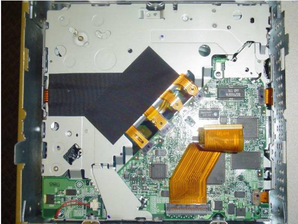
NTG4 REU_Daughterboard
