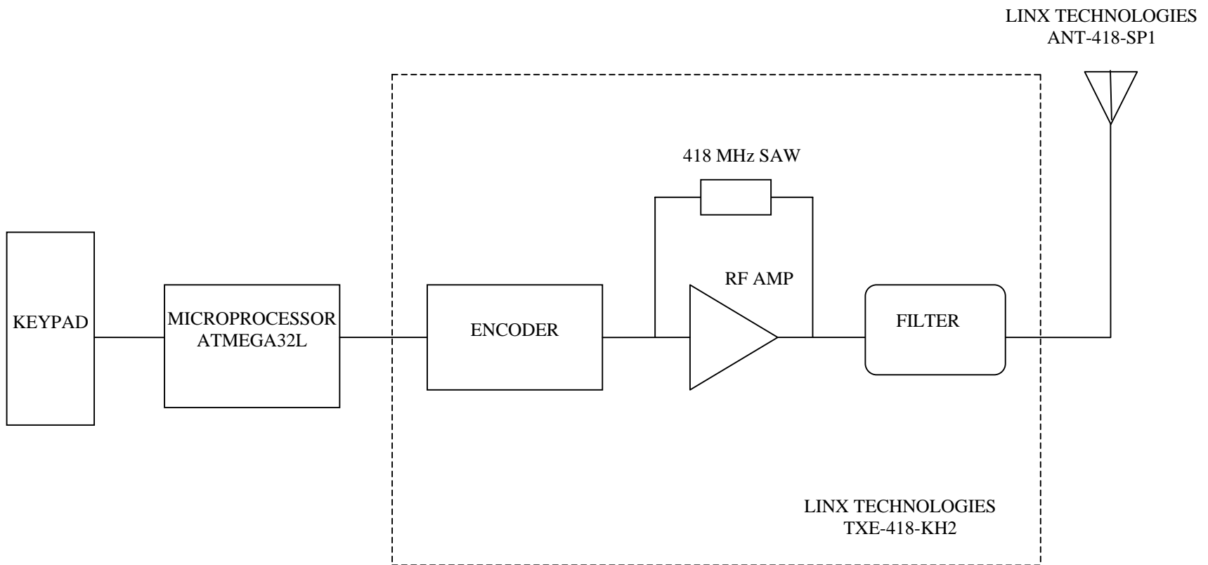
TRANSMITTER BLOCK DIAGRAM
