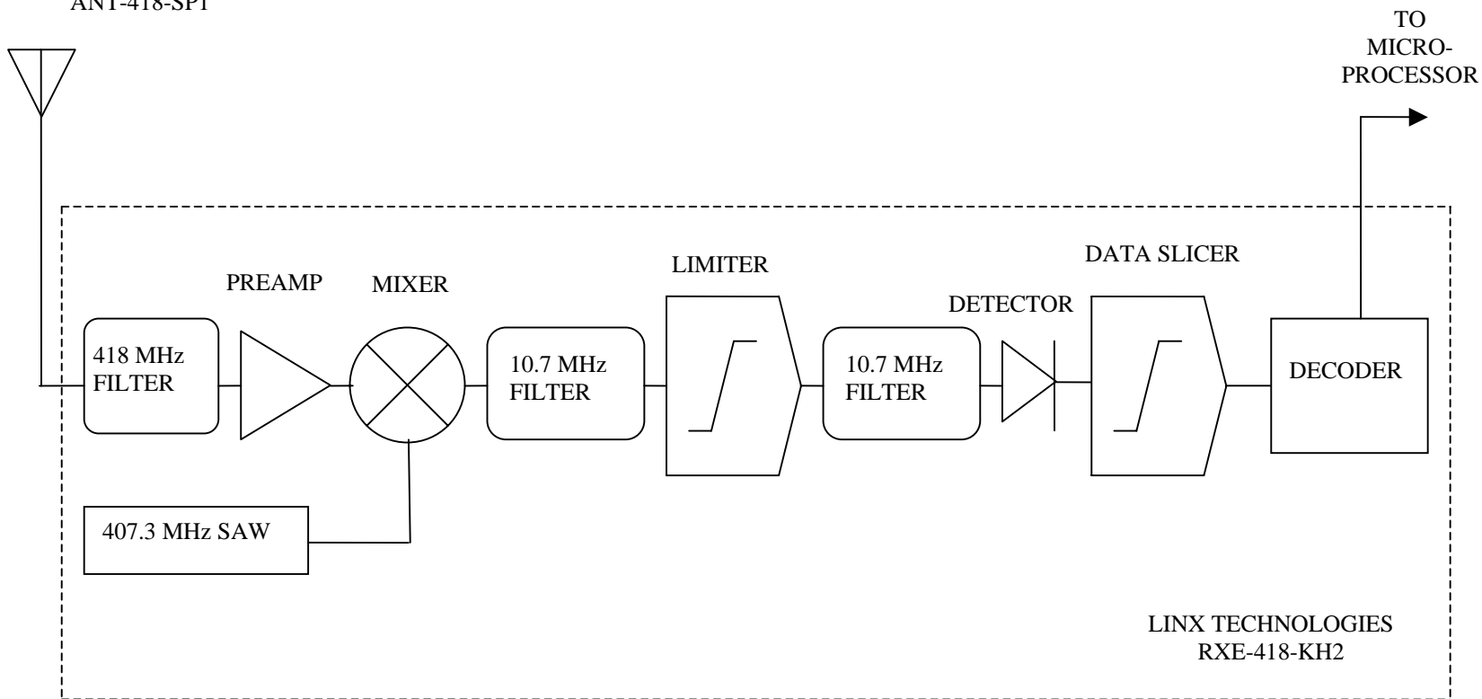
RECEIVER BLOCK DIAGRAM
