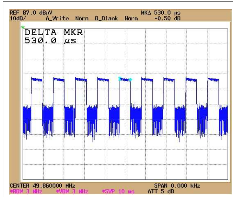
Duty Cycle 3
