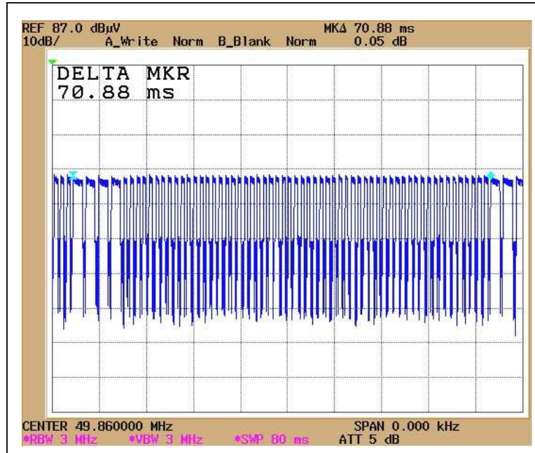
Duty Cycle 1
