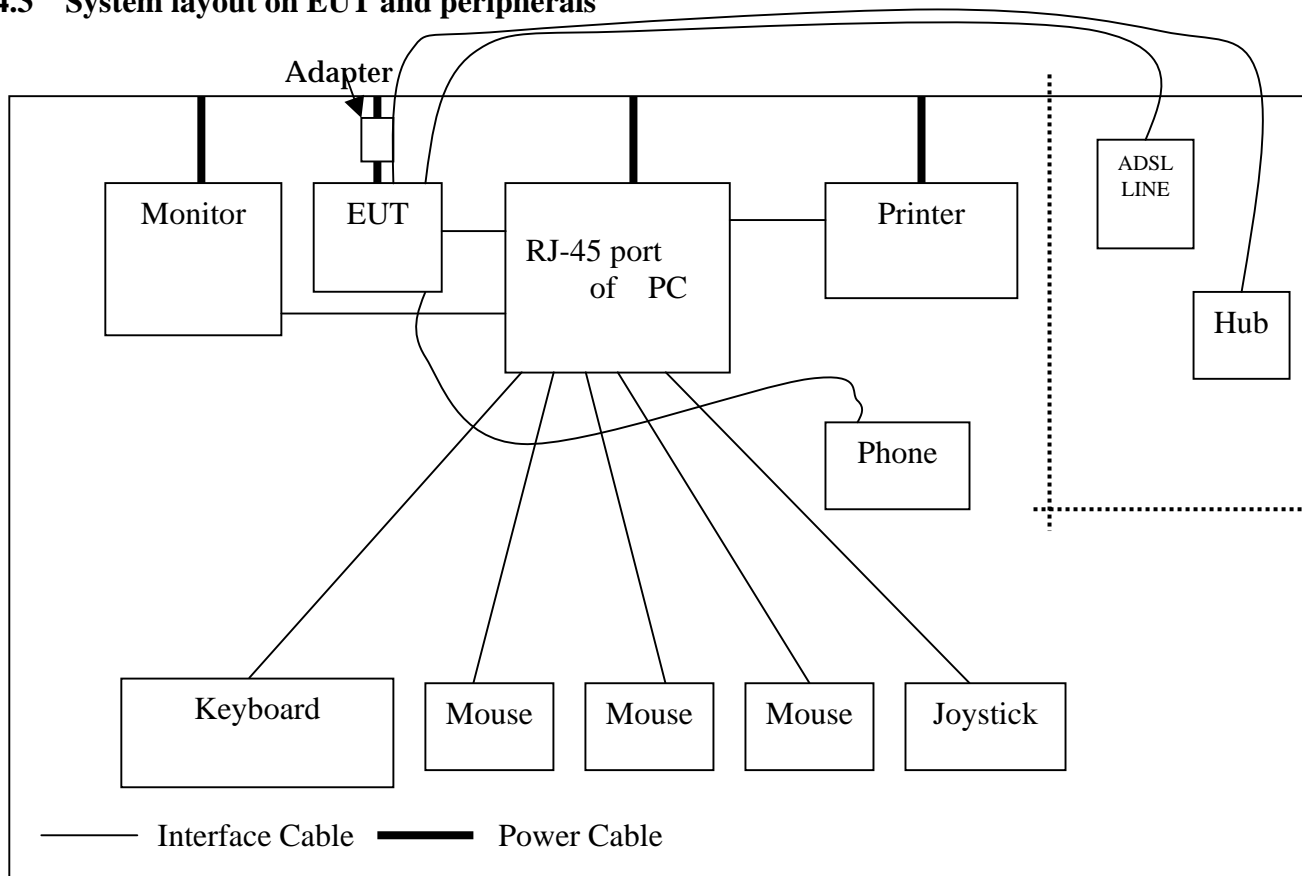
<Figure 4-1 System layout>
